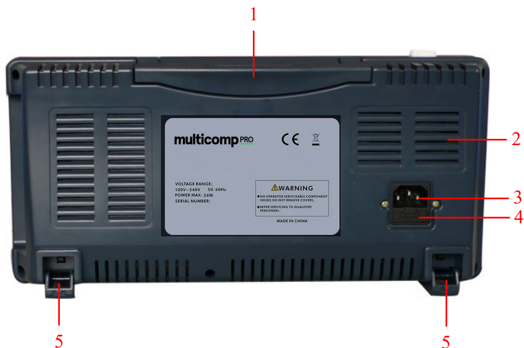
Figure 4-3 Rear Panel
