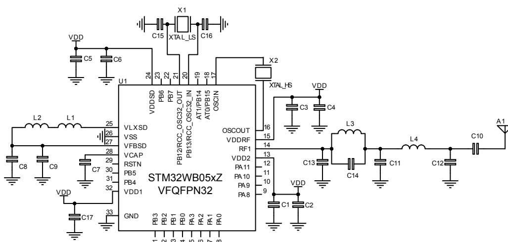
Figure 10. Application circuit: DC-DC converter, VFQFPN32 package
