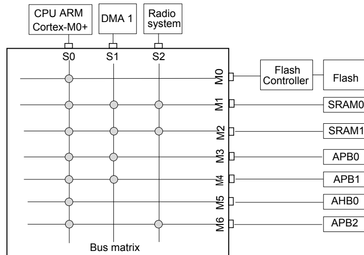
Figure 2. Bus matrix
