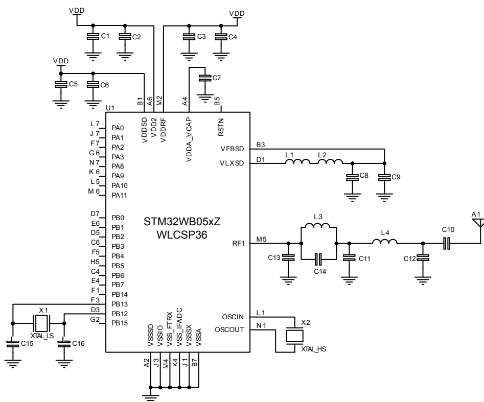
Figure 9. Application circuit: DC-DC converter, WLCSP36 package
