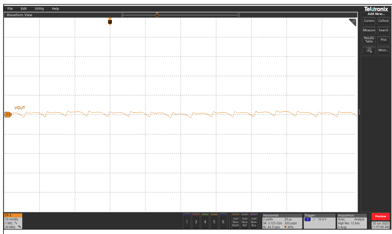
Figure 13 V_{OUT} ripple at 20 A Load, F_{SW} = 800 kHz, (Ch2: V_{OUT} )
