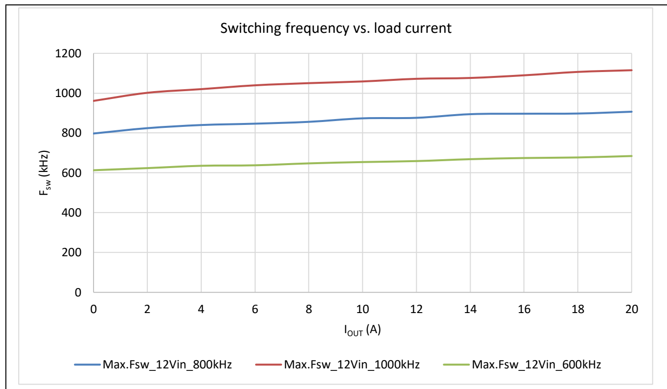
Figure 18 Switching frequency vs. load current
