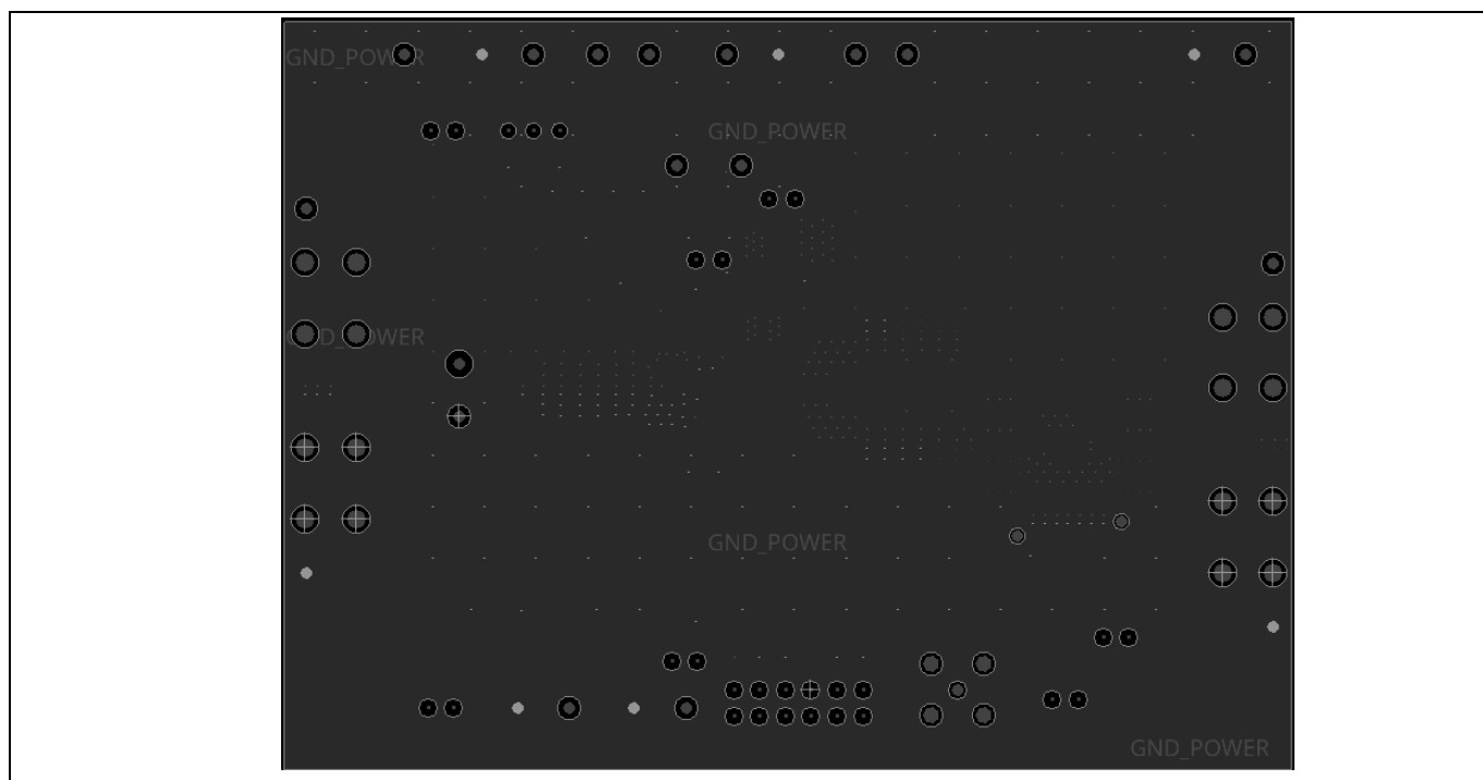
Figure 7 Inner layer 4
