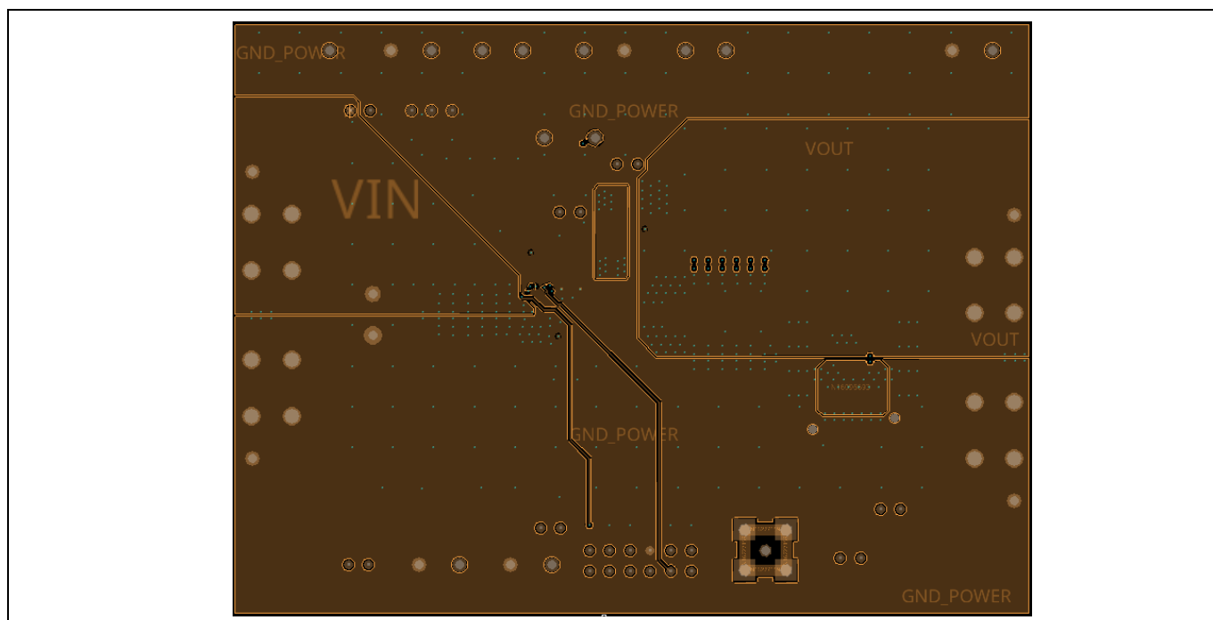
Figure 6 Inner layer 3
