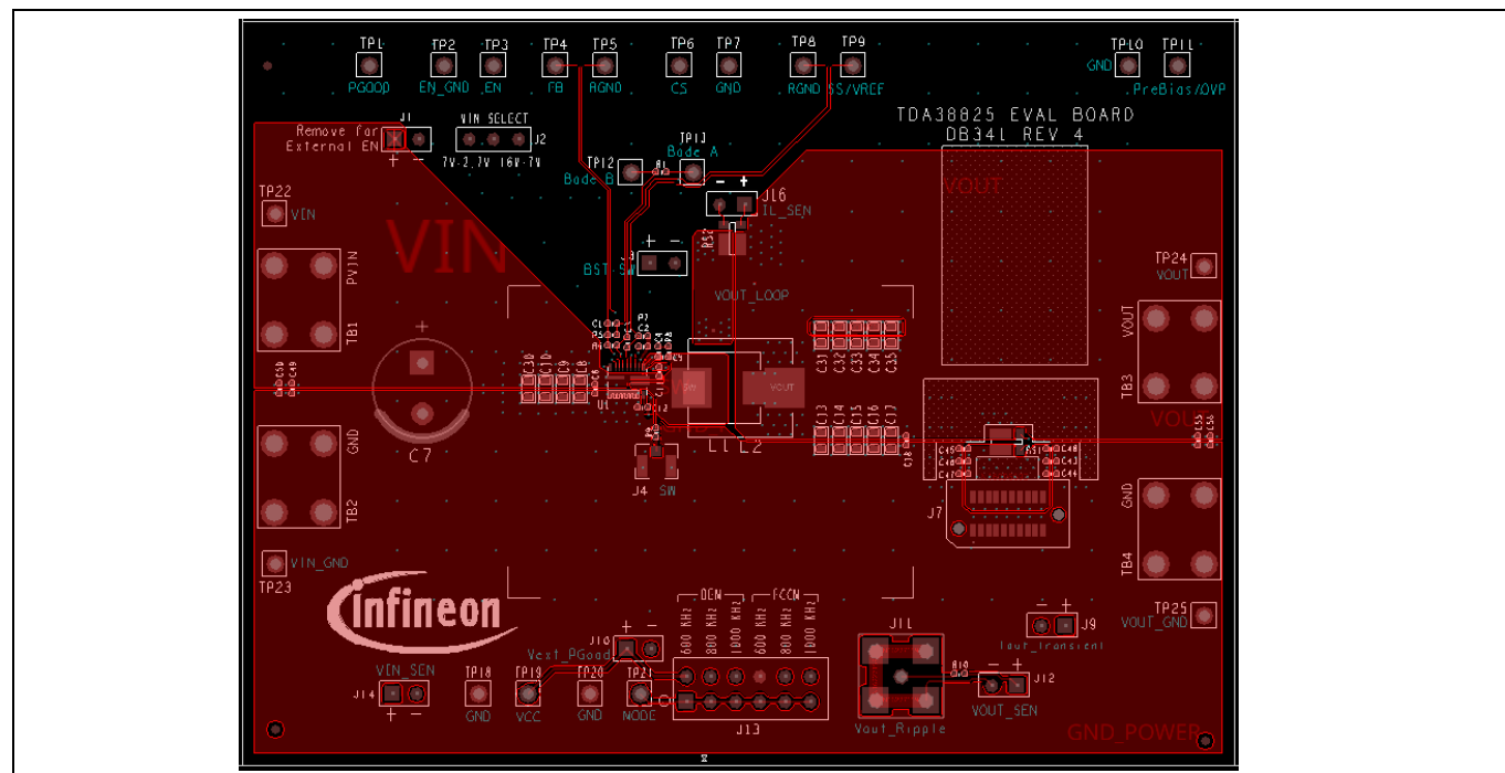
Figure 2 Top layer
