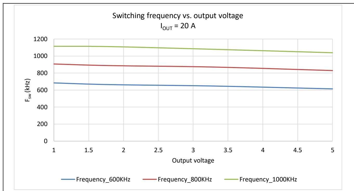
Figure 20 Switching frequency vs. output voltage
