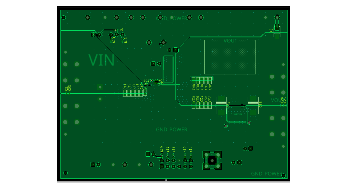
Figure 3 Bottom layer
