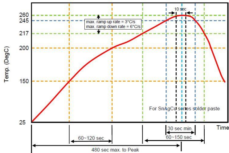
Fig 2. Infrared soldering profile
