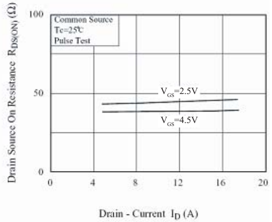
Fig2. R_{DS(on)} - I_D
