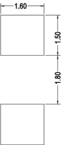
Figure 7: Recommended Soldering Land Pattern
