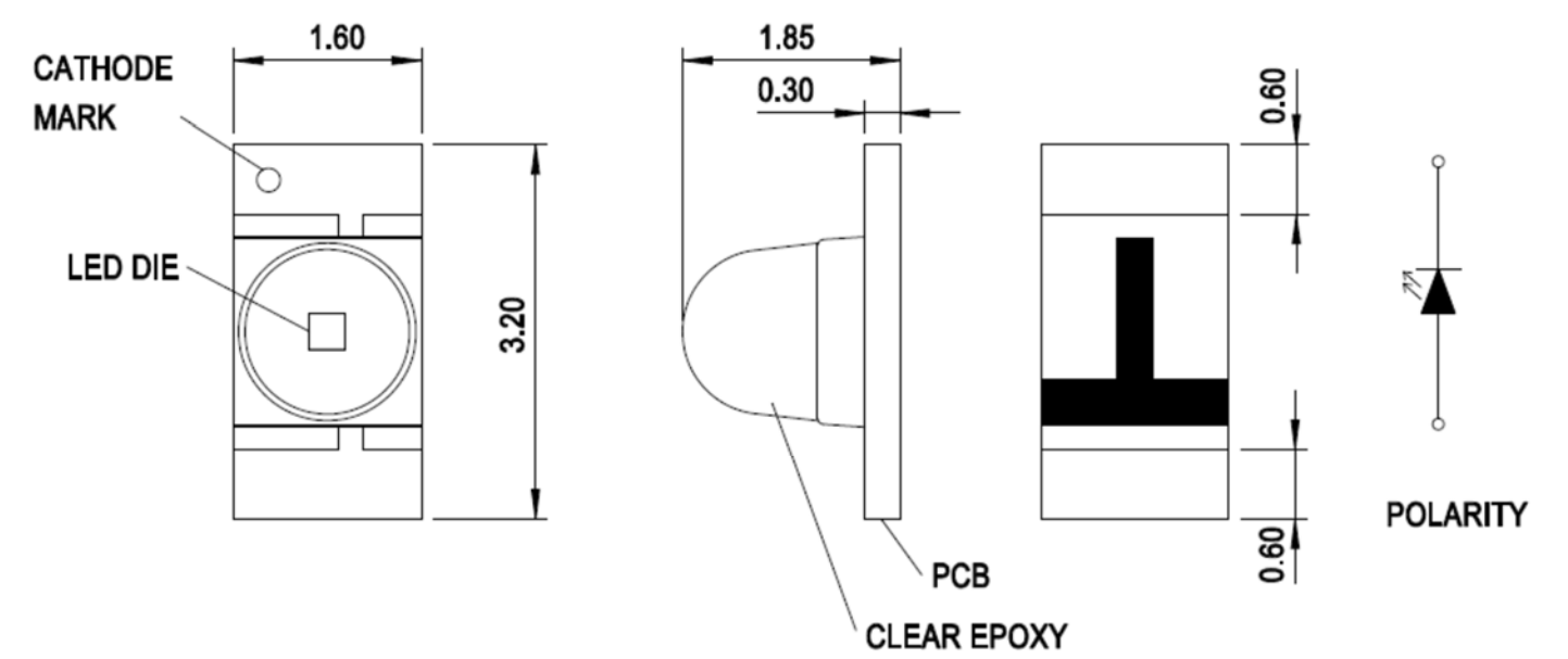
Figure 1: Package Dimensions
