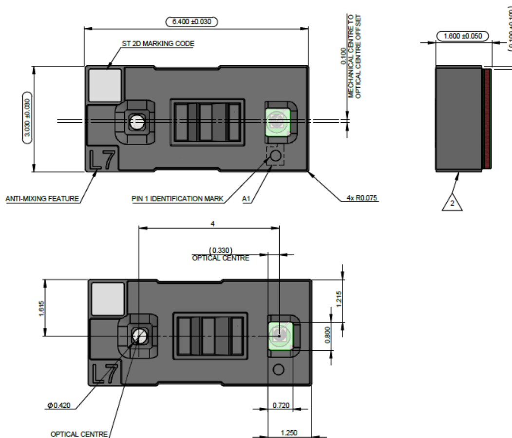
Figure 21. Outline drawing (1/4)
