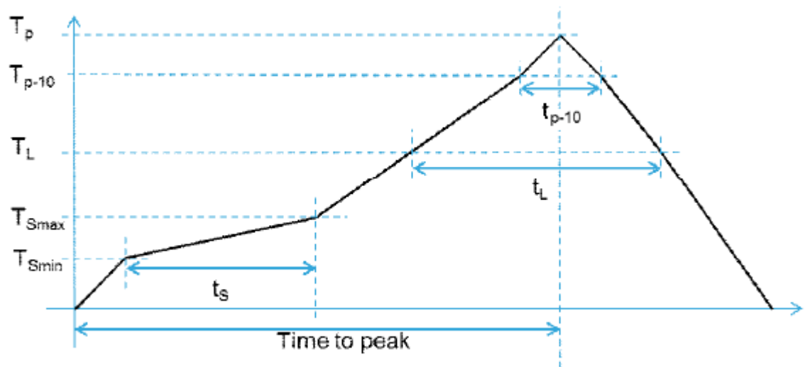
Figure 28. Solder profile
