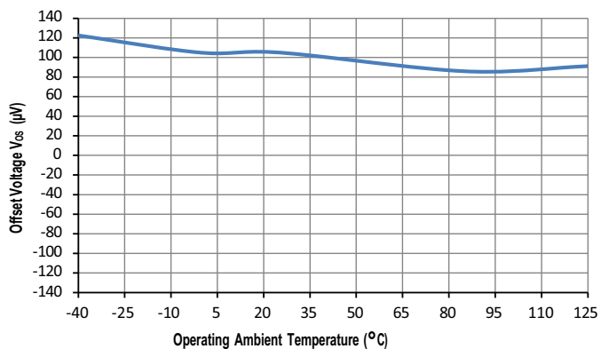
Figure 5: Offset Voltage Change vs. Temperature
