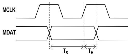
Figure 4: MCLK and MDAT Data Timing
