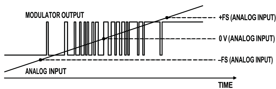
Figure 17: Modulator Output vs. Analog Input
