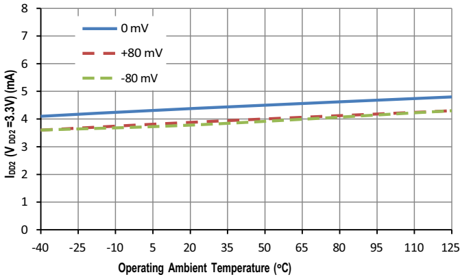
Figure 12: I_{DD2} ( V_{DD2} = 3.3V ) vs. Temperature at Various V_{IN} DC Inputs
