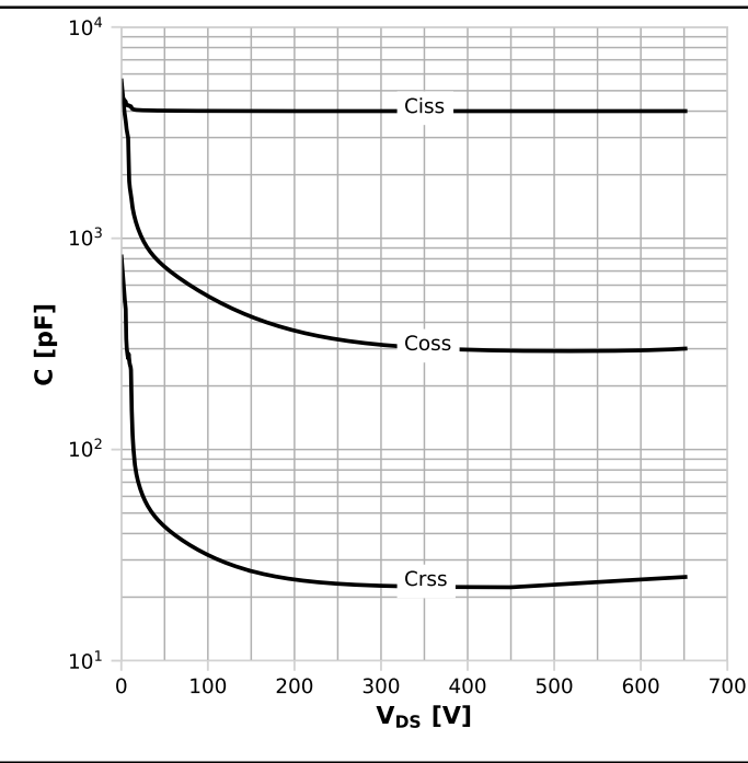
Diagram 15: Typ. capacitances
