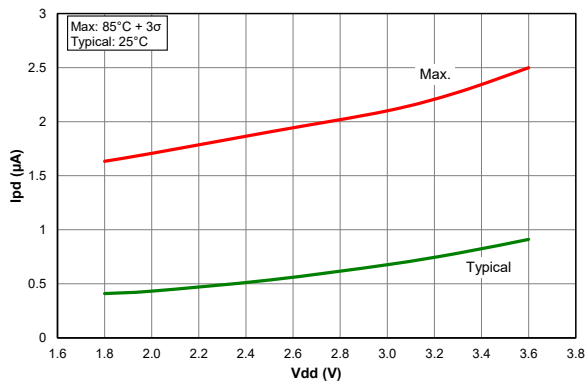
Figure 40-61. I_{PD} , Watchdog Timer, PIC18LF67K40 only
