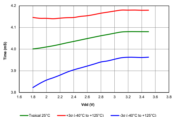
Figure 40-107. Watchdog Timer Time-out Period, PIC18LF67K40 only
