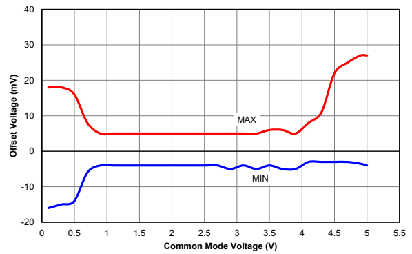
Figure 40-32. Comparator Offset, V_{DD} = 5.5V , from -40°C to 125°C, PIC18F67K40 only
