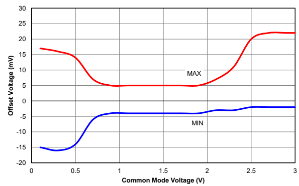
Figure 40-28. Comparator Offset, V DD = 3.0V, from -40°C to 125°C
