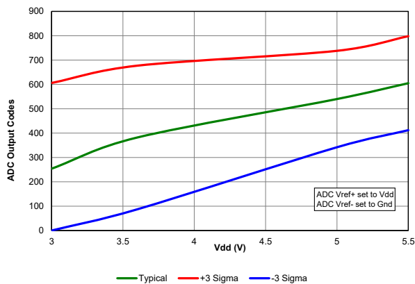
Figure 40-85. Temperature Indicator, Initial Offset, High Range, Temp = 20°C, PIC18F67K40 only
