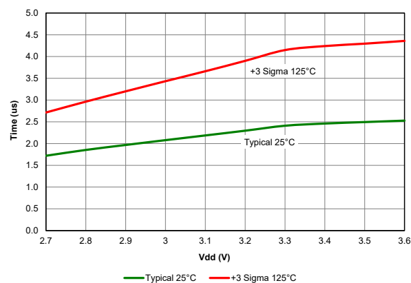
Figure 40-21. BOR Response Time, PIC18LF67K40 only
