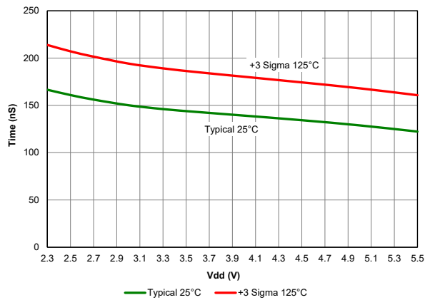
Figure 40-25. Comparator Response Time, Falling Edge, PIC18F67K40 only
