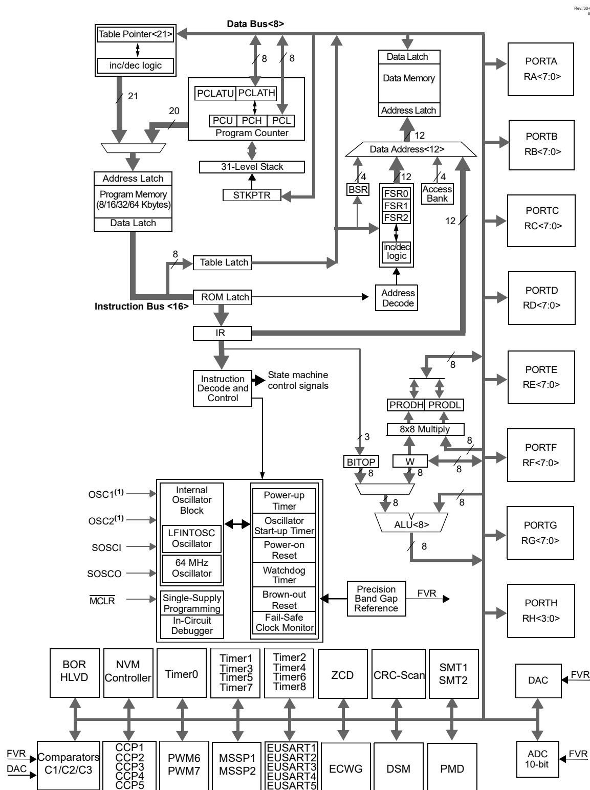
Figure 2-1. PIC18(L)F67K40 Family Block Diagram
