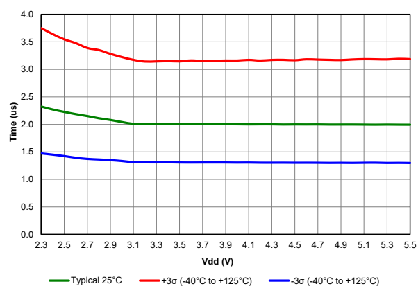
Figure 40-10. ADC RC Oscillator Period, PIC18F67K40 only
