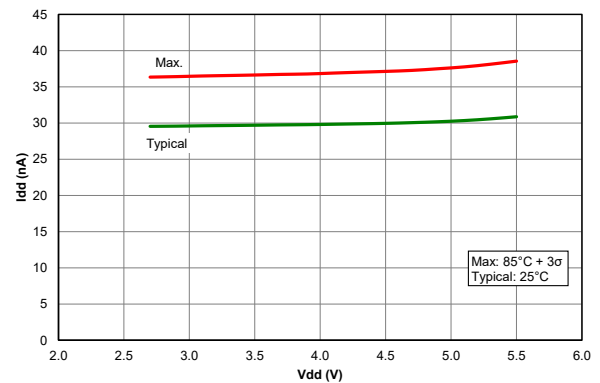
Figure 40-64. I_{DD} , Fixed Voltage Reference (FVR), PIC18F67K40 only
