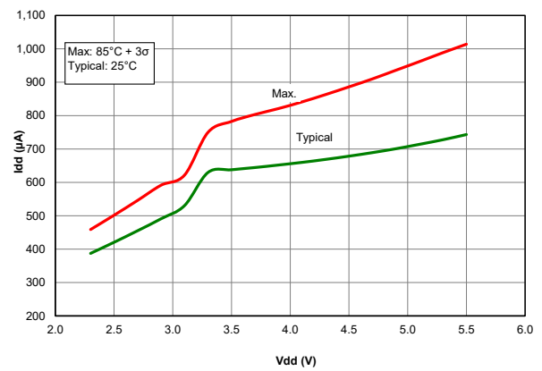
Figure 40-44. I_{DD} , ECM Oscillator, F_{OSC} = 4\text{ MHz} , PIC18F67K40 only
