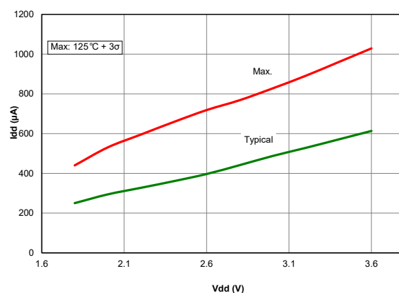
Figure 40-50. I_{DD} , ECM Oscillator, F_{OSC} = 4 MHz, PIC18LF67K40 only
