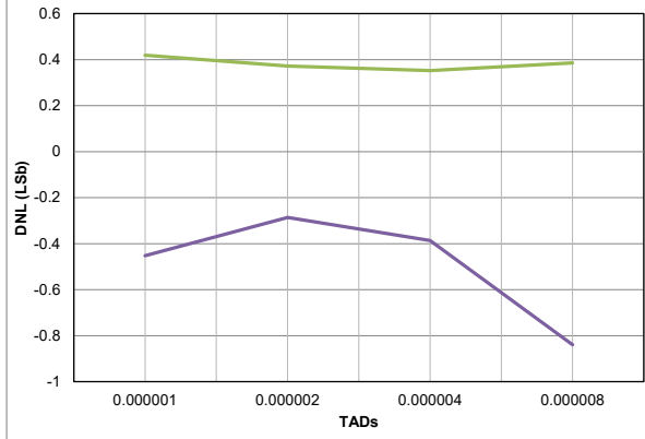
Figure 40-6. ADC, Single-Ended DNL, V_{DD} = 3.0V , V_{REF} = 3.0V
