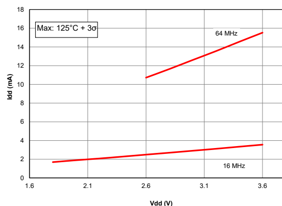
Figure 40-52. I_{DD} , ECH Oscillator, Maximum, PIC18LF67K40 only
