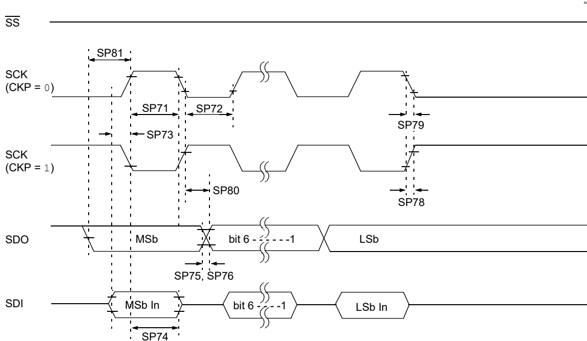
Figure 39-17. SPI Host Mode Timing (CKE = 1, SMP = 1)
