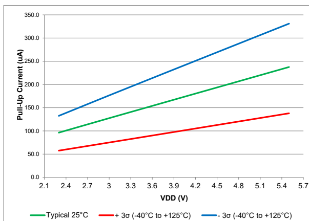
Figure 40-108. Weak Pull-up Current, PIC18F67K40 only
