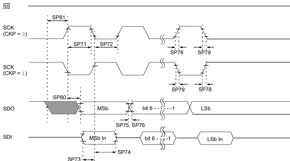
Figure 39-16. SPI Host Mode Timing (CKE = 0, SMP = 0)
