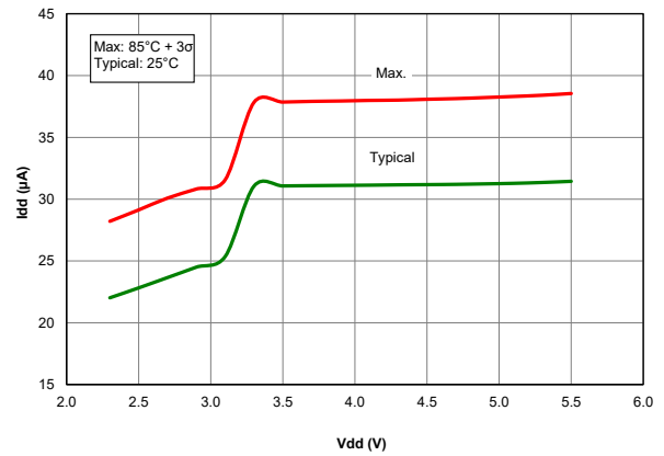
Figure 40-42. I_{DD} , LFINTOSC, F_{OSC} = 31\text{ kHz} , PIC18F67K40 only
