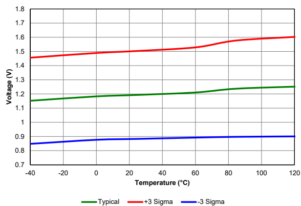
Figure 40-81. POR Rearm Voltage, VREGPM1 = 1, PIC18F67K40 only
