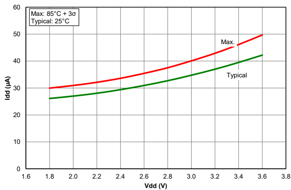
Figure 40-63. I_{DD} , Fixed Voltage Reference (FVR), PIC18LF67K40 only
