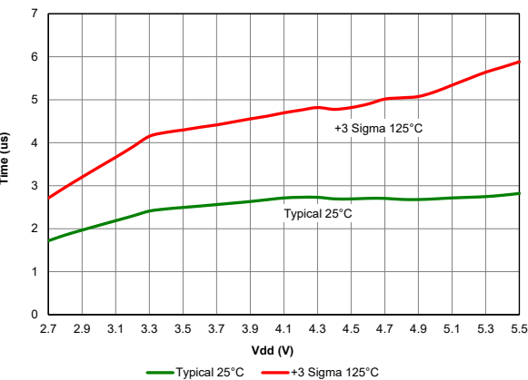
Figure 40-22. BOR Response Time, PIC18F67K40 only
