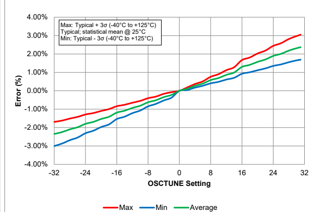
Figure 40-78. OSTUNE Center Frequency
