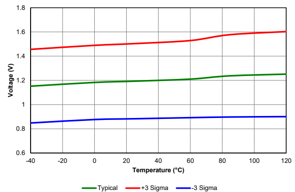
Figure 40-82. POR Rearm Voltage, Normal Power Mode, PIC18LF67K40 only
