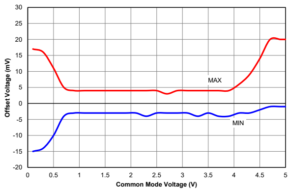
Figure 40-31. Comparator Offset, V_{DD} = 5.0V , 25°C, PIC18F67K40 only
