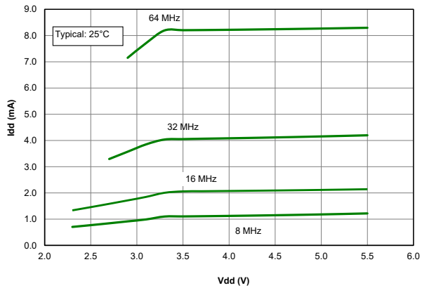
Figure 40-45. I_{DD} , ECH Oscillator, Typical, PIC18F67K40 only
