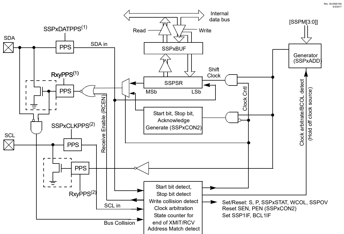
Figure 28-9. MSSP Block Diagram (I 2 C Host Mode)
