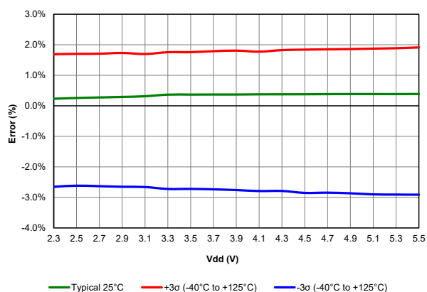
Figure 40-40. HFINTOSC Typical Frequency Error, PIC18F67K40 only
