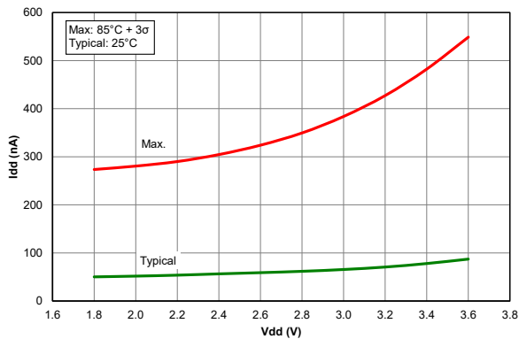
Figure 40-71. I_{PD} Base, Low-power Sleep Mode, PIC18LF67K40 only
