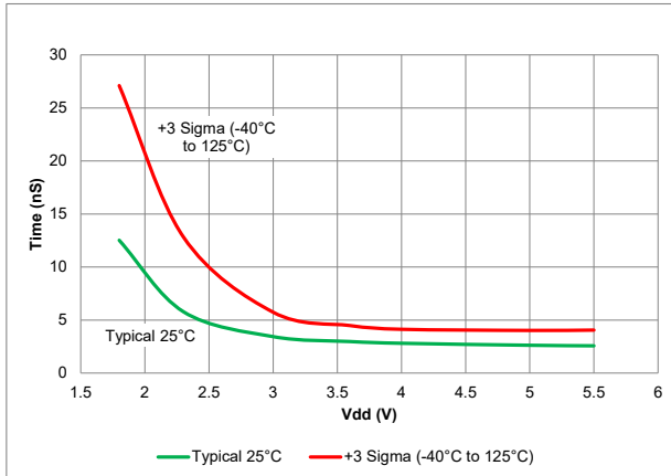
Figure 40-59. I/O Rise Time, Slew Rate Control Disabled
