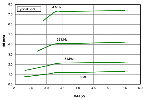
Figure 39-45. I_{DD} , ECH Oscillator, Typical, PIC18F27/47K40 only
