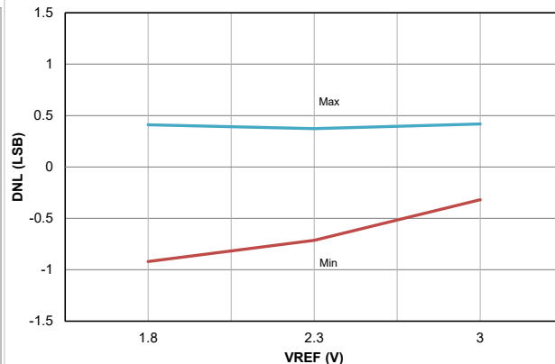
Figure 39-8. ADC, Single-Ended DNL, V_{DD} = 3.0V , T_{AD} = 1 \mu S
