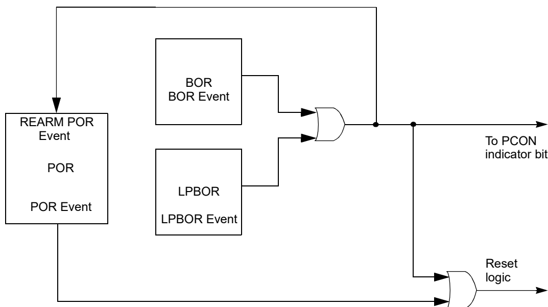
Figure 9-3. LPBOR, BOR, POR Relationship
