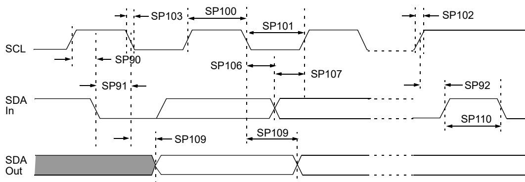
Figure 38-21. I 2 C Bus Data Timing
