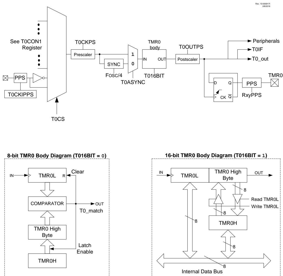
Figure 19-1. Timer0 Block Diagram
