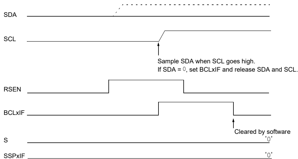
Figure 27-37. Bus Collision During a Repeated Start Condition (Case 1)
