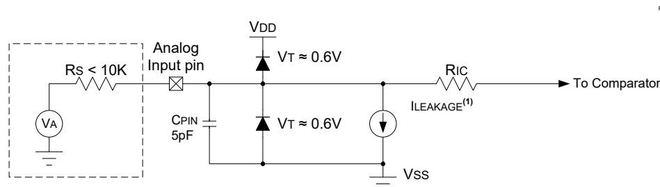
Figure 33-3. Analog Input Model
