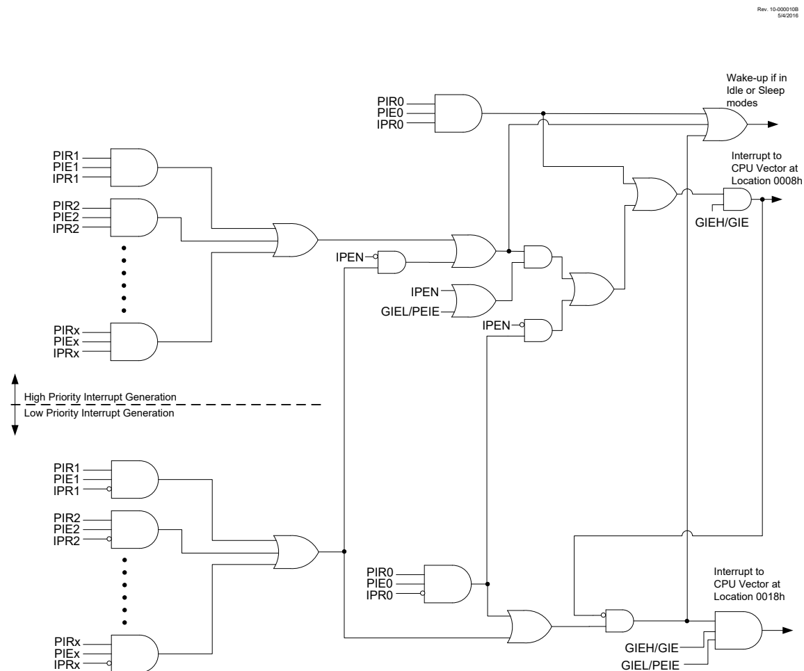
Figure 15-1. PIC18 Interrupt Logic
