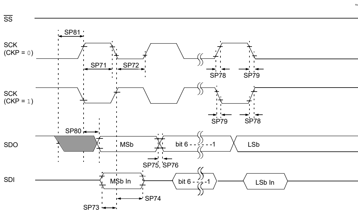
Figure 38-16. SPI Host Mode Timing (CKE = 0, SMP = 0)
