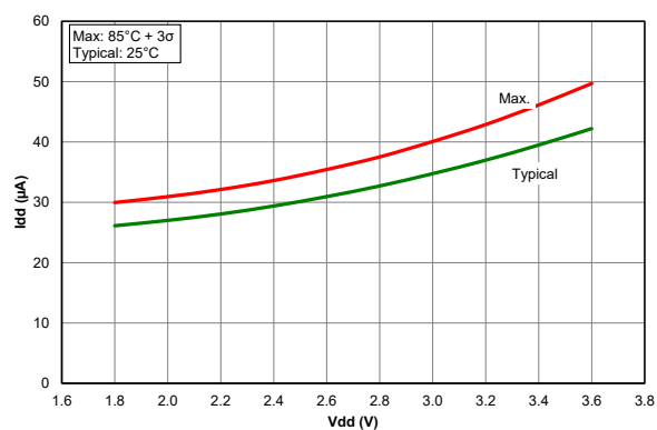
Figure 39-63. I_{PD} , Fixed Voltage Reference (FVR), PIC18LF27/47K40 only
