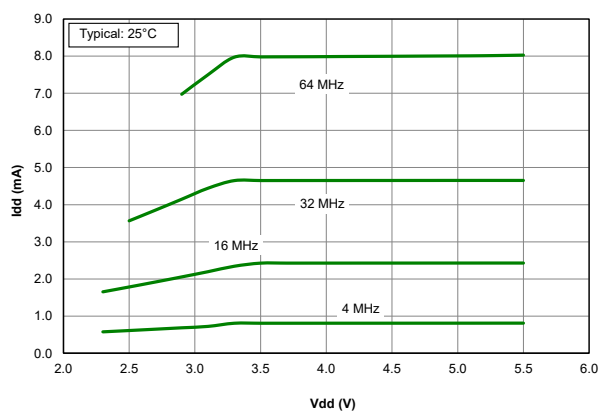
Figure 39-47. I_{DD} , HFINTOSC, Typical, PIC18F27/47K40 only
