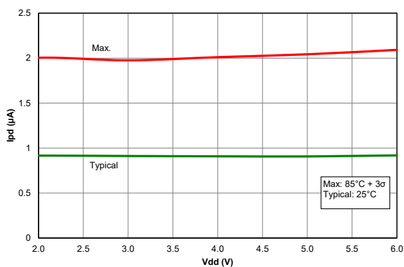
Figure 39-62. I_{PD} , Watchdog Timer, PIC18F27/47K40 only
