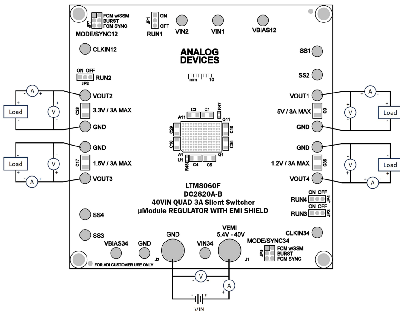
Figure 2. Test Setup of DC2820A-B
