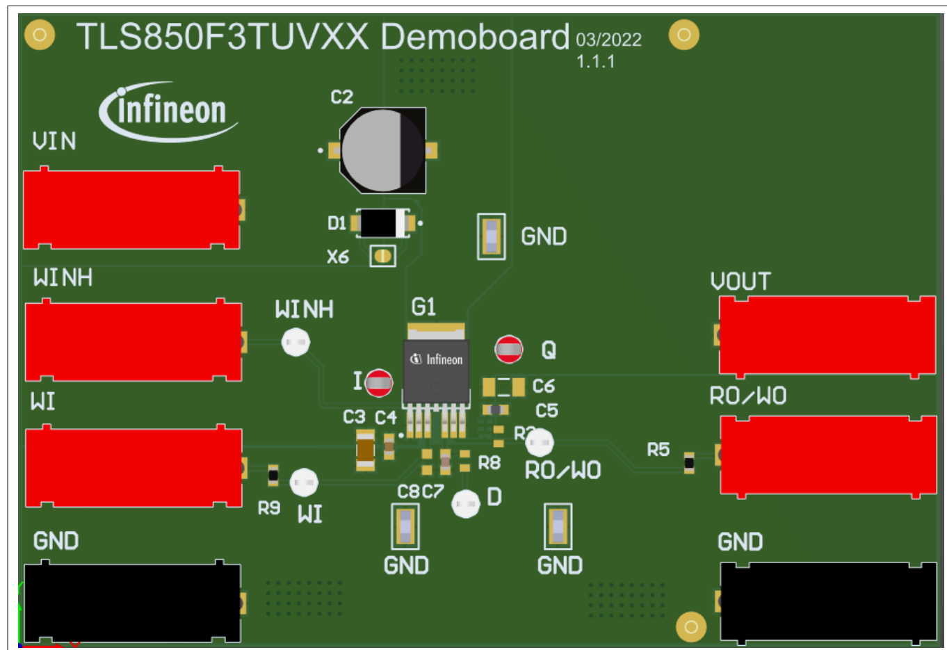
Figure 2 Assembly TLS850F3TUVxx demoboard
