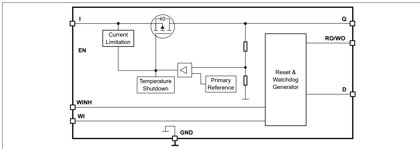
Figure 1 Block diagram TLS850F3TUVxx
