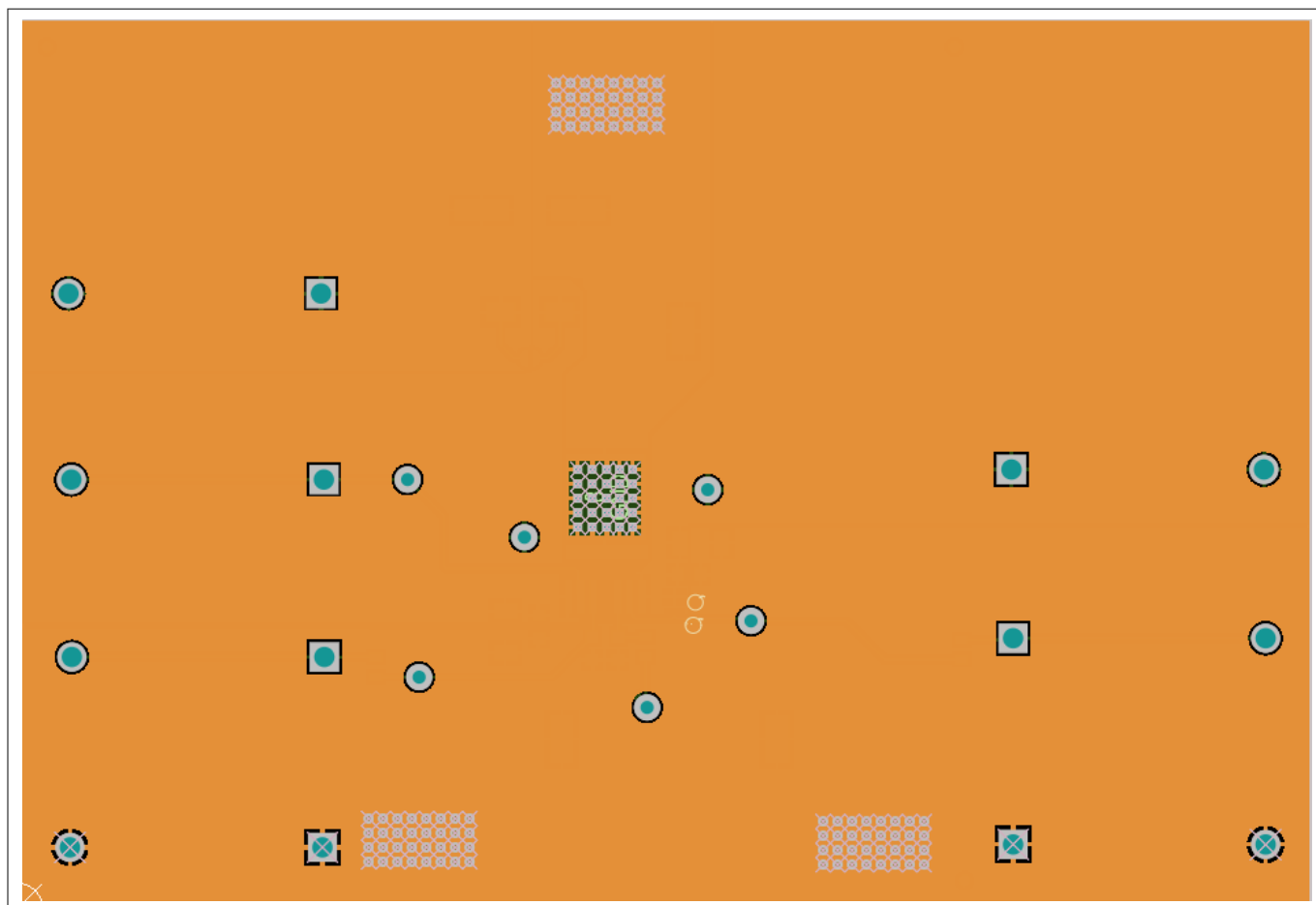
Figure 6 Bottom layer TLS850F3TUVxx demoboard
