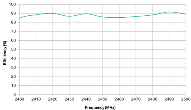
2.4 GHz Efficiency
