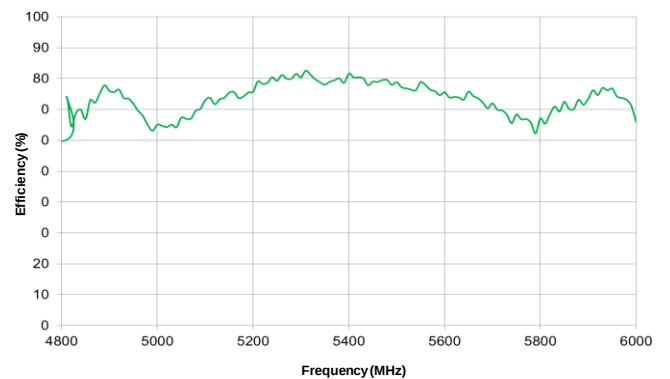
5 GHz Efficiency
