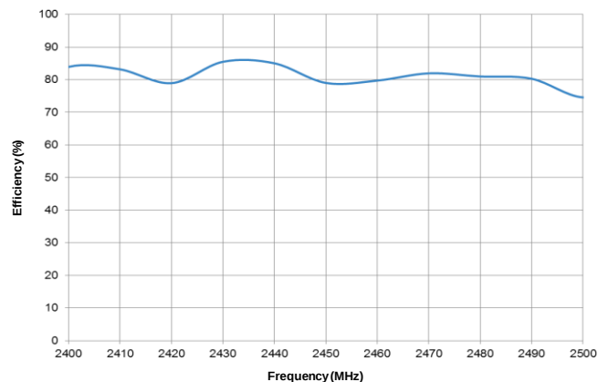
2.4 GHz Efficiency
