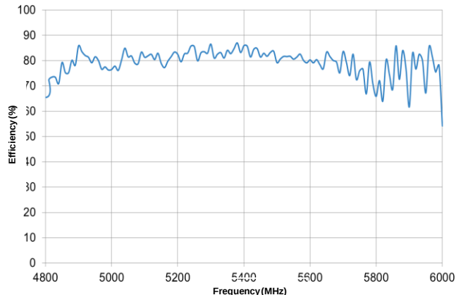
5 GHz Efficiency
