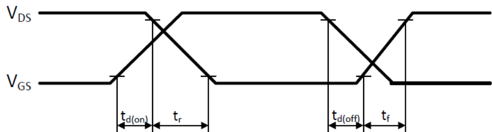
Figure 1-20. Switching Waveform
