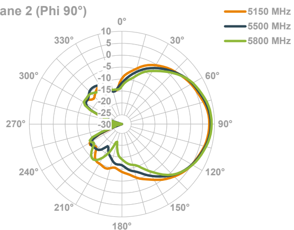
El. Plane 2 (Phi 90°)
