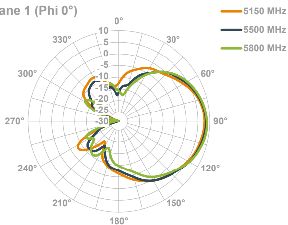
El. Plane 1 (Phi 0°)
