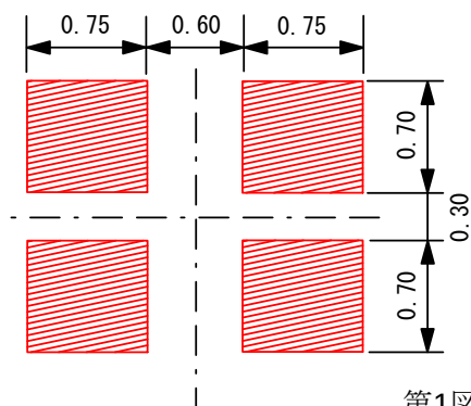
Figure 1. Dimensions
