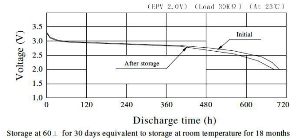
Storage characteristic
