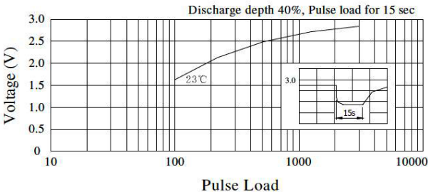
Pulse discharge characteristic
