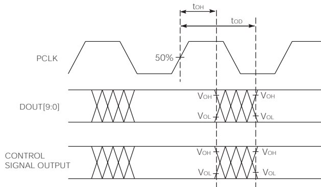
Figure 3-14: PCLK to Data & Control Signal Output Timing
