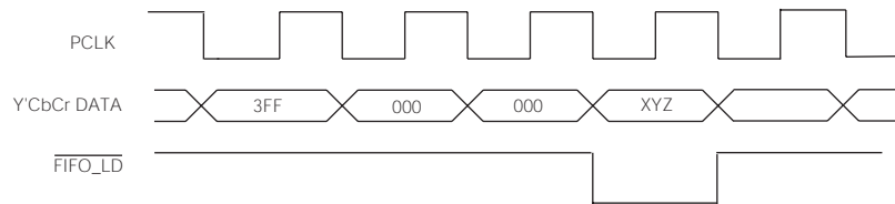
Figure 3-6: FIFO_LD Pulse Timing
