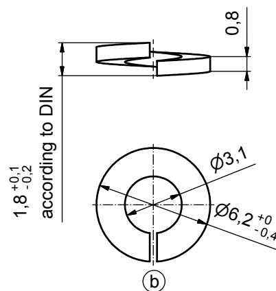
SPRING RING
