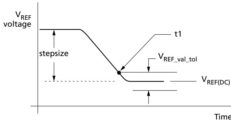
Figure 105: V_{REF(DQ)} Full Step from V_{REF,min} to V_{REF,max}
