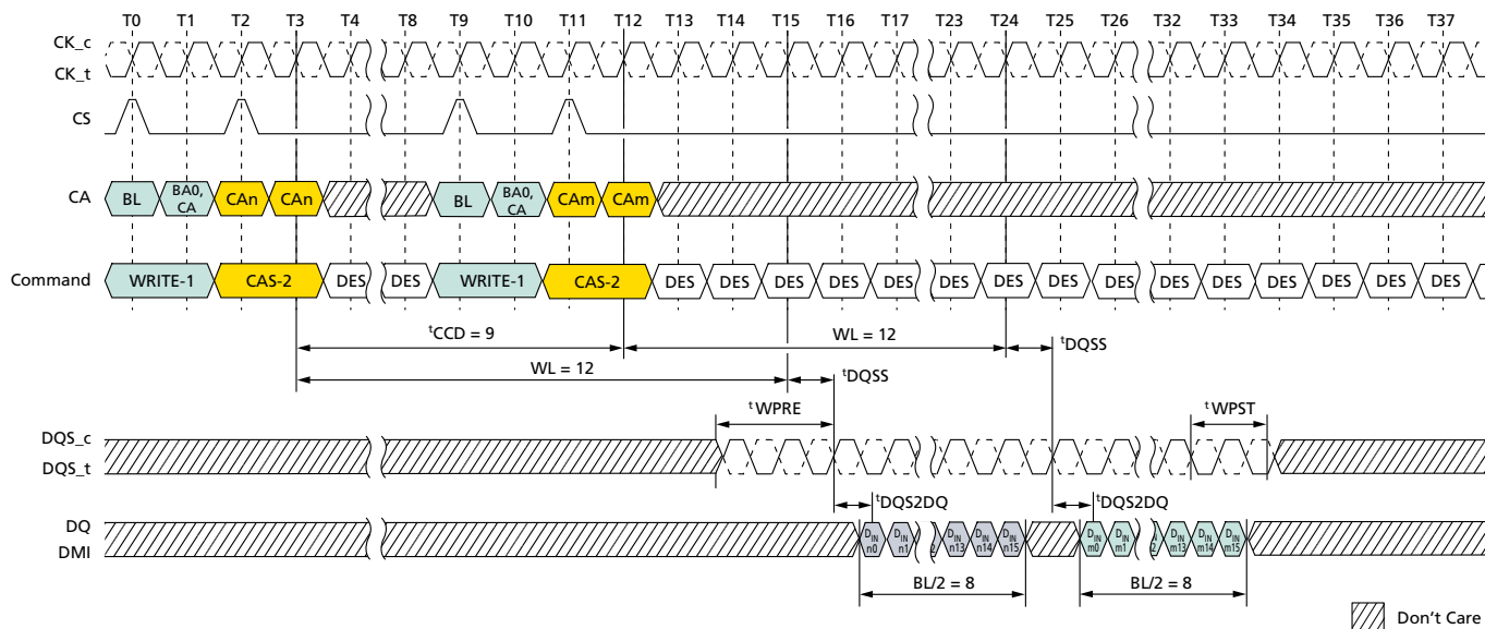
Figure 51: Consecutive WRITE: t_{CCD} = MIN + 1, 1.5nCK Postamble
