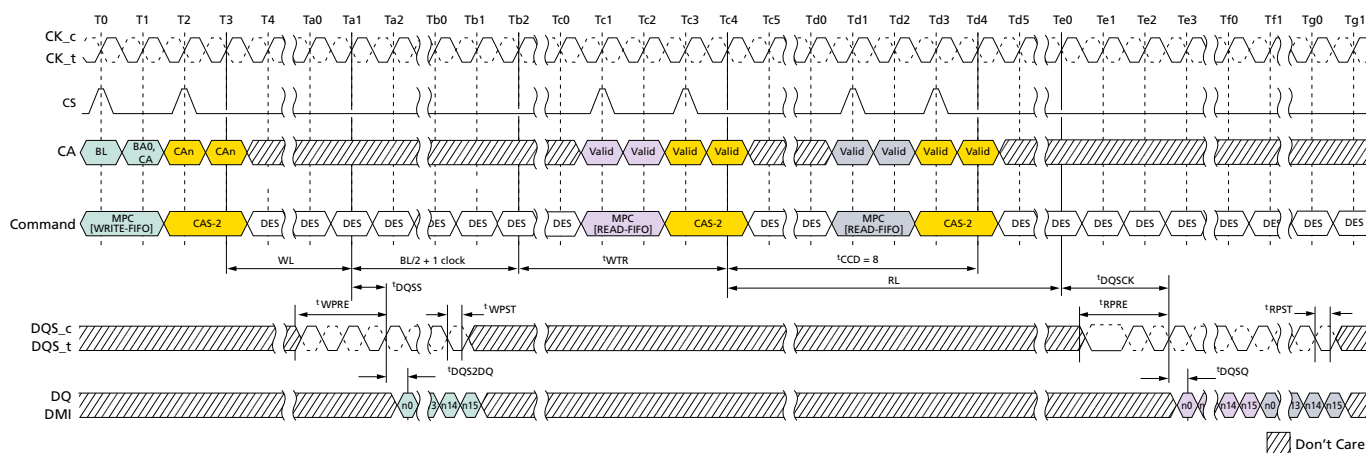
Figure 122: MPC[WRITE-FIFO]-to-MPC[READ-FIFO] Timing
