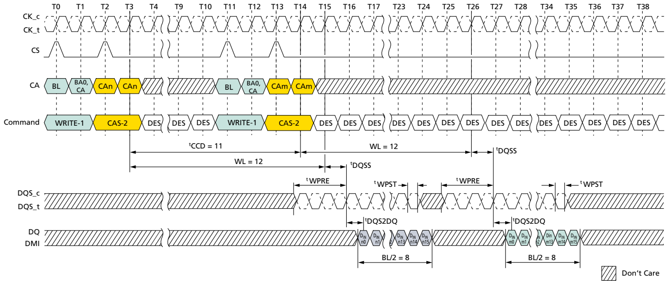
Figure 54: Consecutive WRITE: t_{CCD} = \text{MIN} + 3, 0.5nCK Postamble
