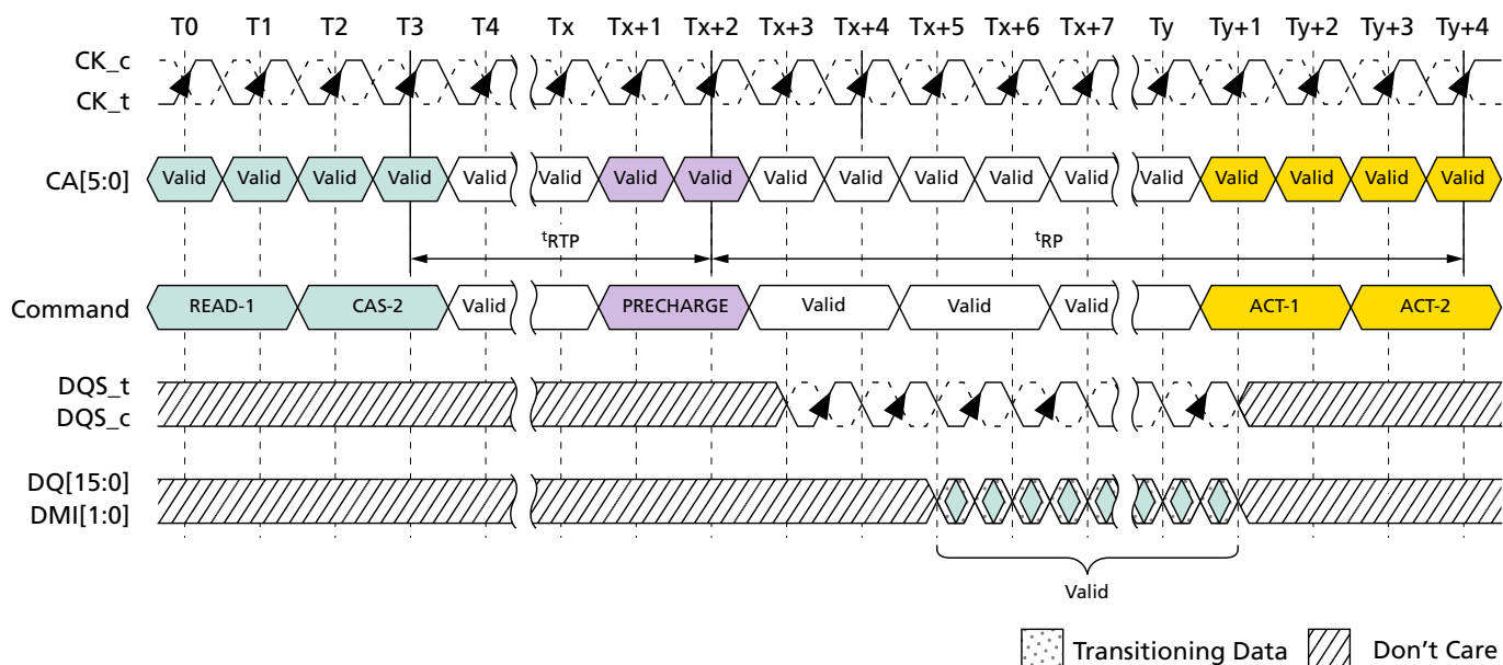
Figure 58: Burst READ Followed by Precharge – BL32, 2 t CK, 0.5nCK Postamble
