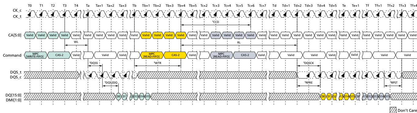
Figure 116: READ-FIFO – t_{WPST} = 2nCK , t_{WPST} = 0.5nCK , t_{RPRE} = \text{Toggling} , t_{RPST} = 1.5nCK
