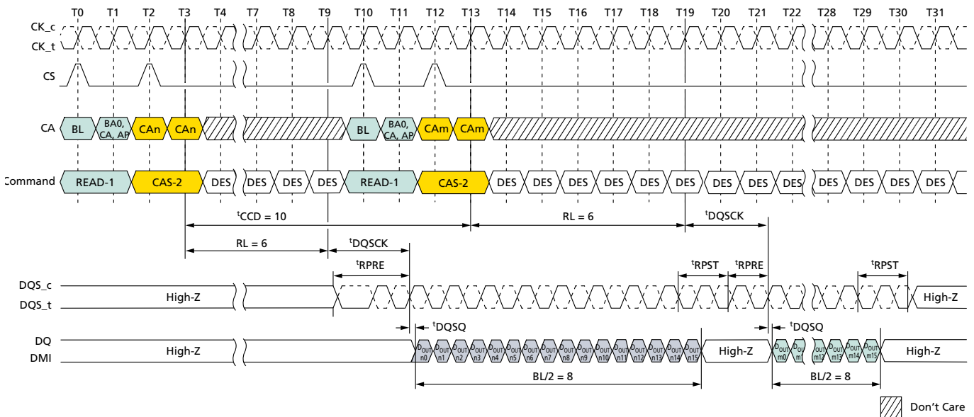
Figure 39: Consecutive READ: t_{CCD} = \text{MIN} + 2 , Preamble = Toggle, 1.5n\text{CK} Postamble
