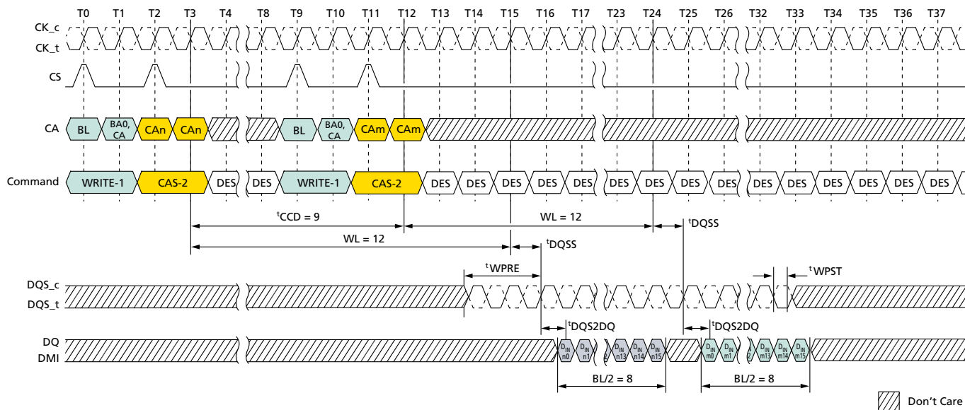
Figure 50: Consecutive WRITE: t_{CCD} = MIN + 1, 0.5nCK Postamble
