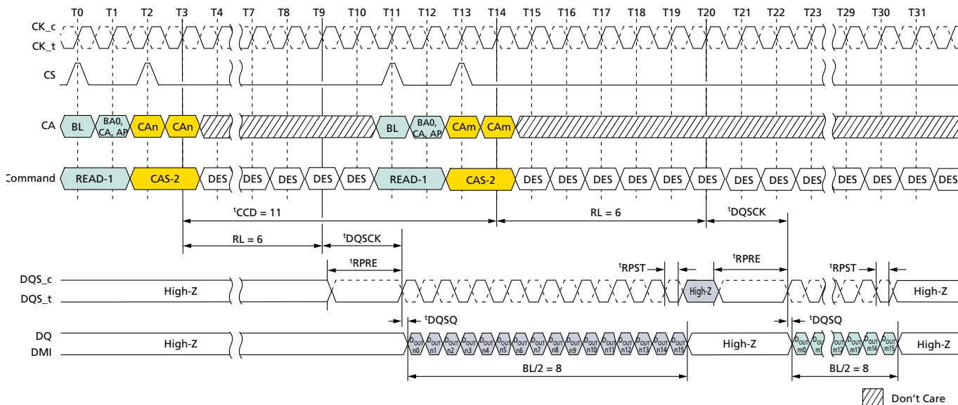
Figure 46: Consecutive READ: t_{CCD} = \text{MIN} + 3 , Preamble = Static, 0.5n\text{CK} Postamble
