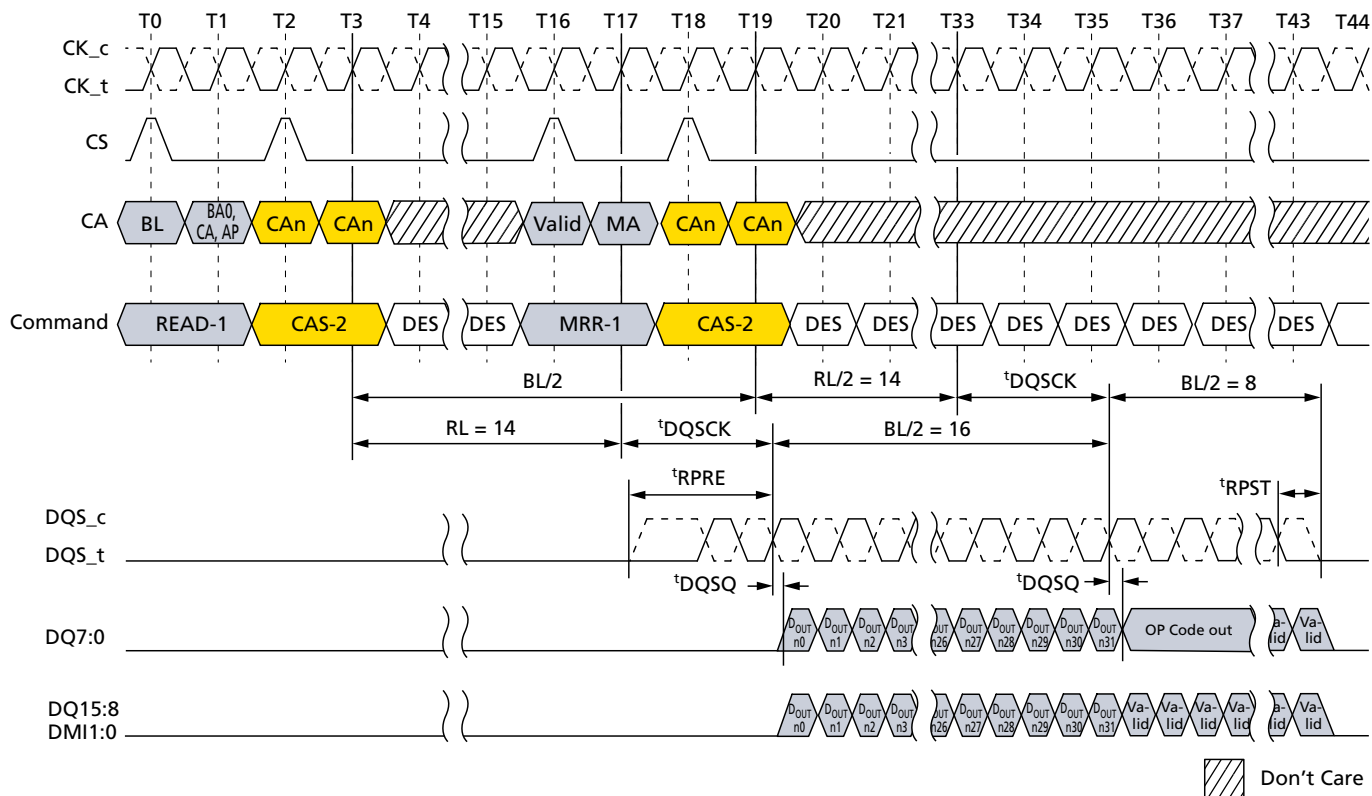
Figure 87: READ-to-MRR Timing
