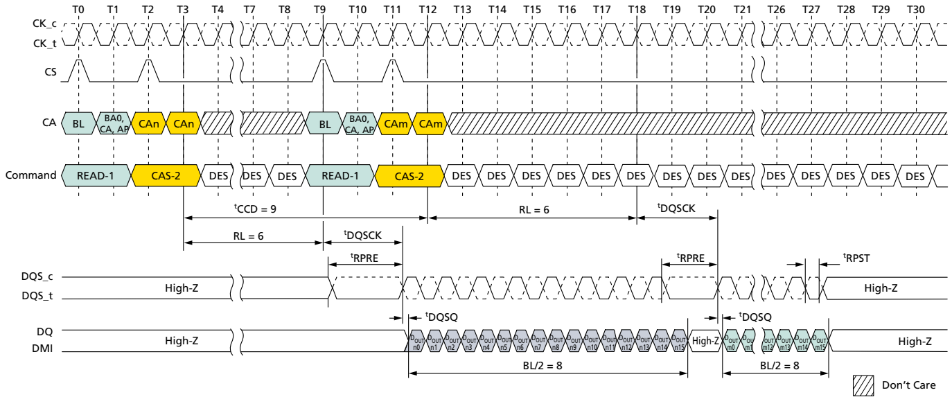
Figure 38: Consecutive READ: t_{CCD} = \text{MIN} + 1 , Preamble = Static, 0.5n\text{CK} Postamble
