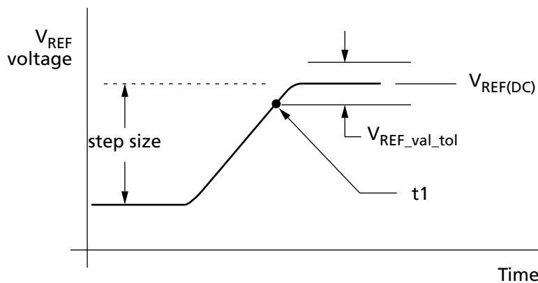
Figure 96: V REF(CA) Single-Step Increment
