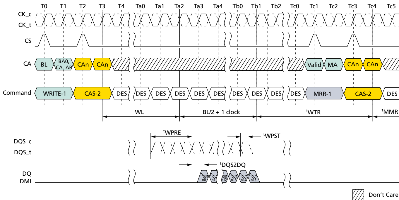
Figure 88: WRITE-to-MRR Timing
