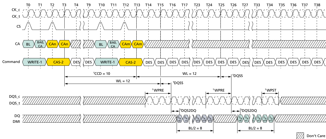
Figure 53: Consecutive WRITE: t_{CCD} = MIN + 2, 1.5nCK Postamble
