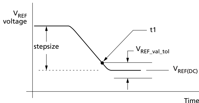
Figure 98: V REF(CA) Full Step from V REF,min to V REF,max
