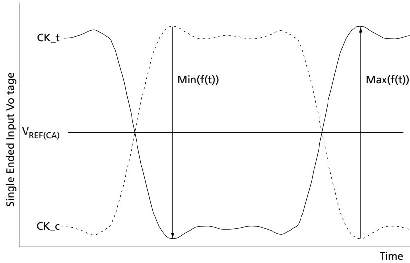
Figure 145: Definition of Differential Clock Peak Voltage
