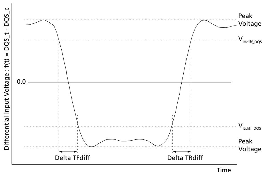
Figure 152: Differential Input Slew Rate Definition for DQS t , DQS c
