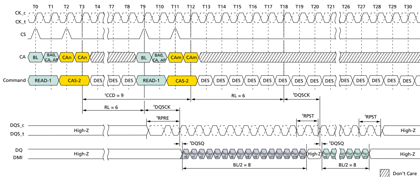
Figure 35: Seamless READ: t_{CCD} = \text{MIN} + 1 , Preamble = Toggle, 1.5n\text{CK} Postamble
