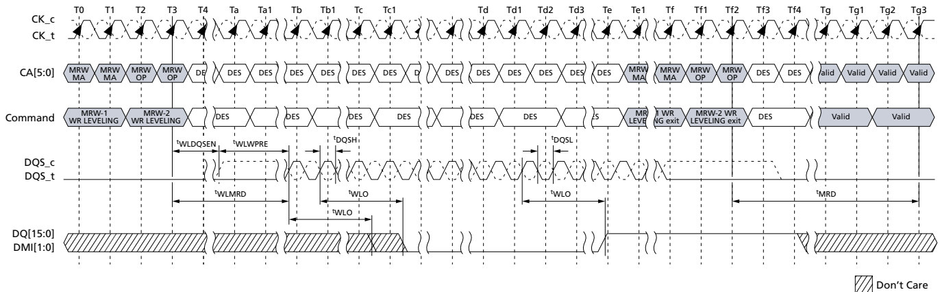
Figure 112: Write Leveling Timing – t_{DQSL}(\text{MIN})
