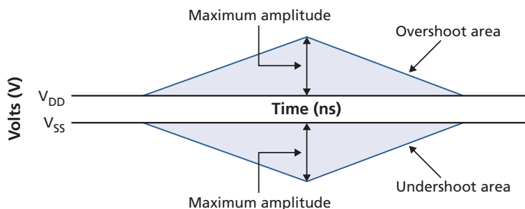
Figure 156: Overshoot and Undershoot Definition
