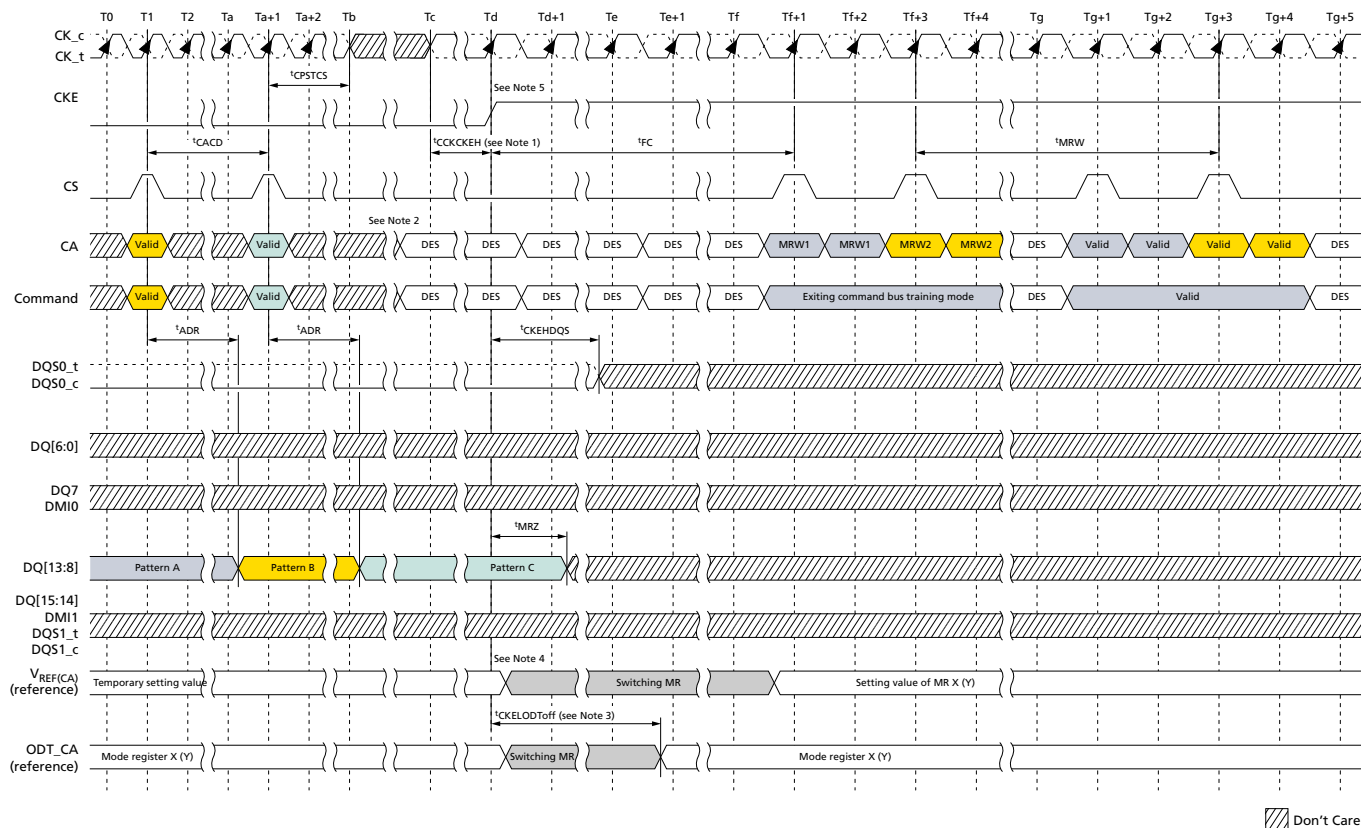
Figure 109: Command Bus Training Mode Exit with Valid Command
