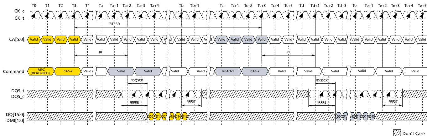
Figure 117: READ-FIFO – t_{RPRE} = \text{Toggling} , t_{RPST} = 1.5nCK
