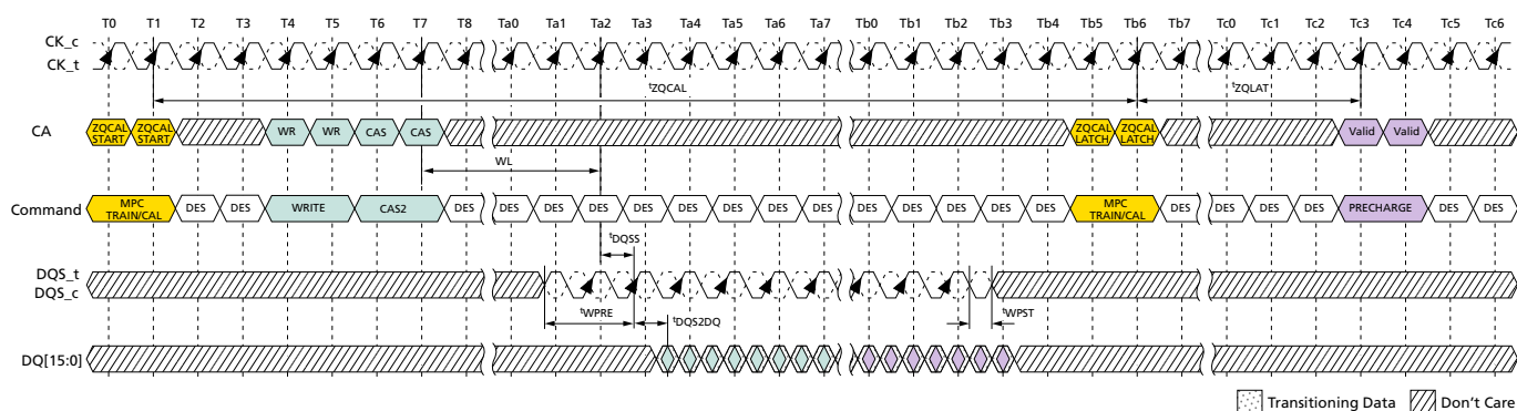
Figure 130: ZQCAL Timing
