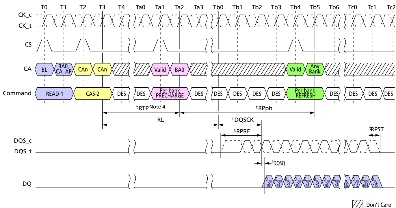
Figure 69: Burst READ Operation Followed by Per-Bank Refresh
