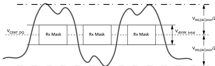
Figure 172: DQ V_{IHL(AC)} Definition (for Each Input Pulse)
