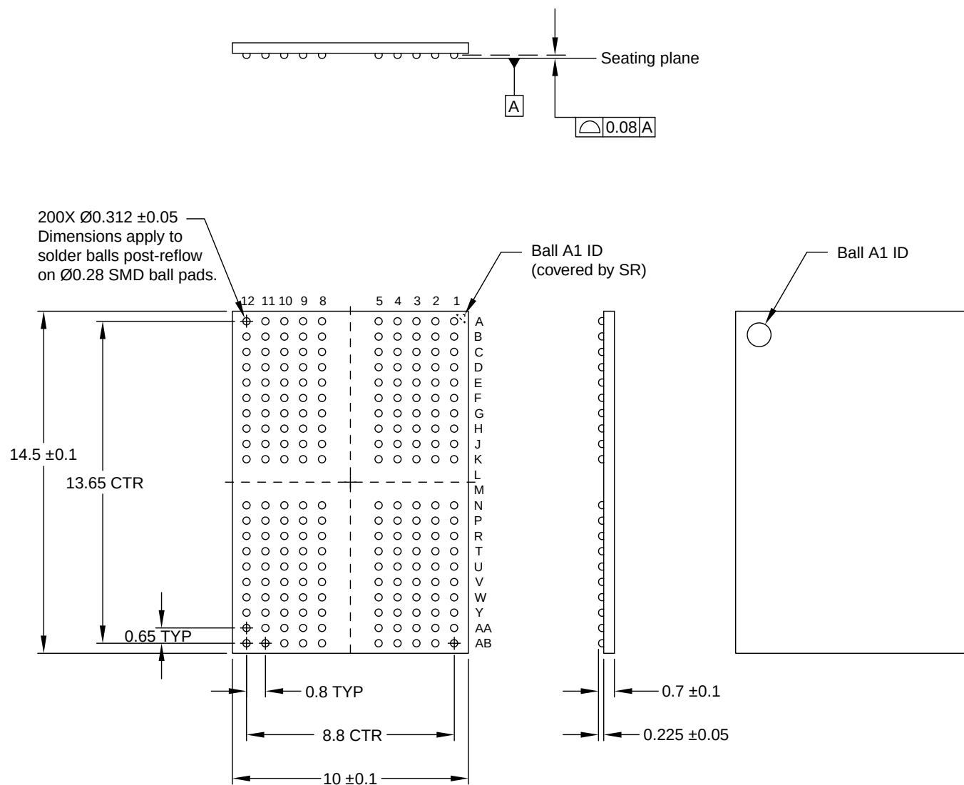
Figure 5: 200-Ball WFBGA – 10mm x 14.5mm (Package Code: NP)
