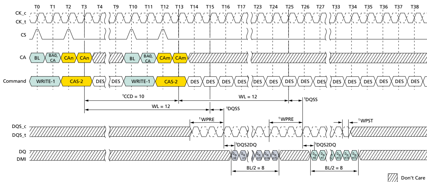
Figure 52: Consecutive WRITE: t_{CCD} = MIN + 2, 0.5nCK Postamble
