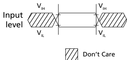
Figure 143: Input Timing Definition for RESET_n
