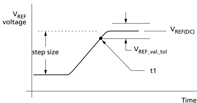
Figure 103: V REF(DQ) Single-Step Size Increment
