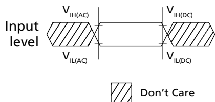
Figure 142: Input Timing Definition for CKE
