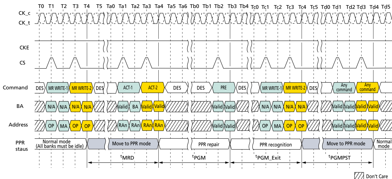
Figure 140: Post-Package Repair Timing
