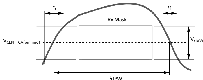
Figure 165: CA t_{cIPW} and SRIN_cIVW Definition (for Each Input Pulse)
