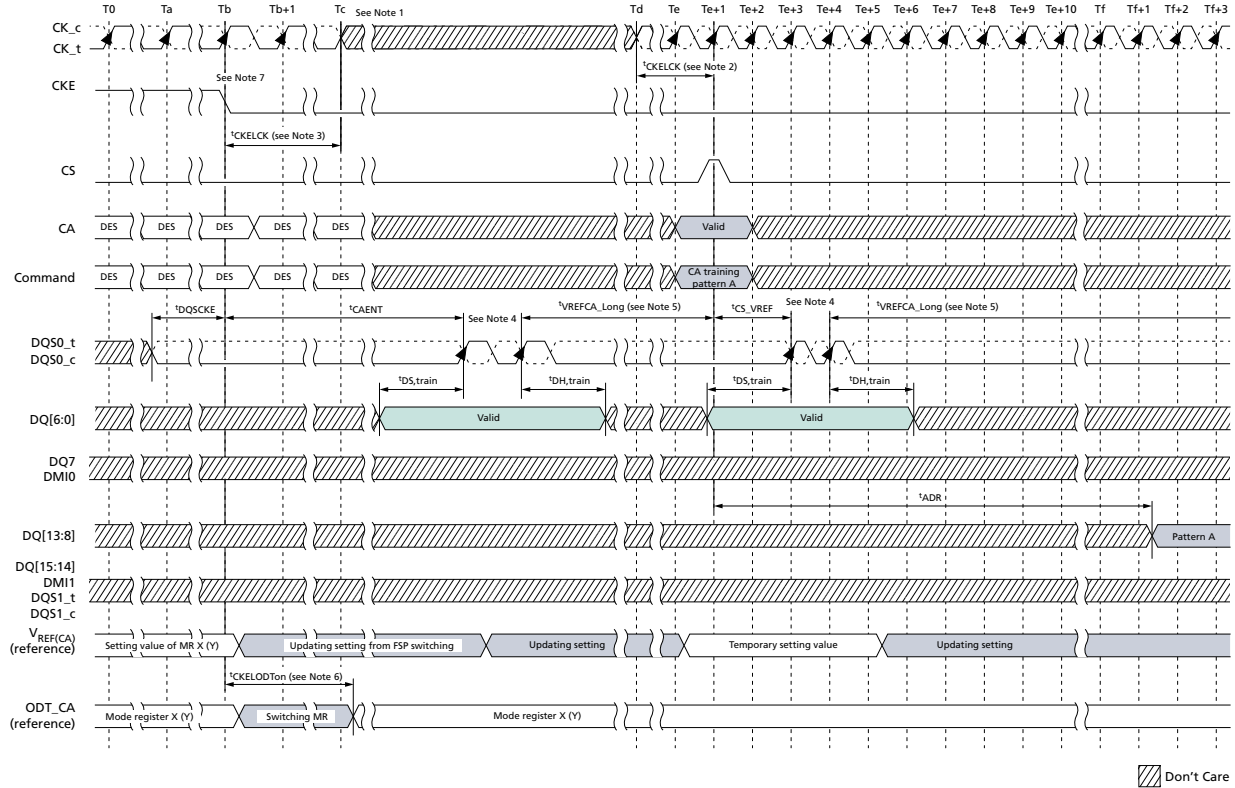
Figure 108: Consecutive V_{REF(CA)} Value Update
