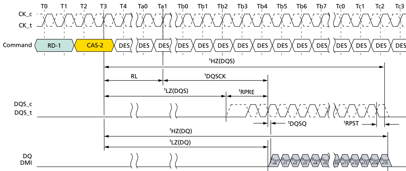
Figure 20: Read Timing
