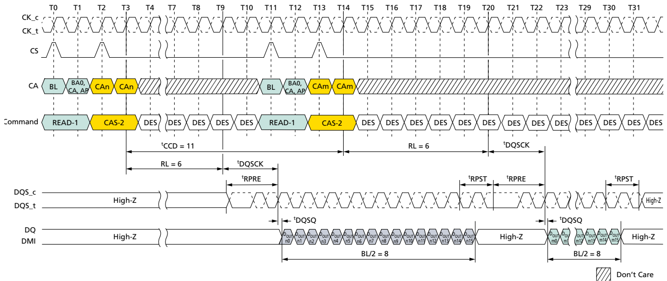
Figure 43: Consecutive READ: t_{CCD} = \text{MIN} + 3 , Preamble = Toggle, 1.5n\text{CK} Postamble
