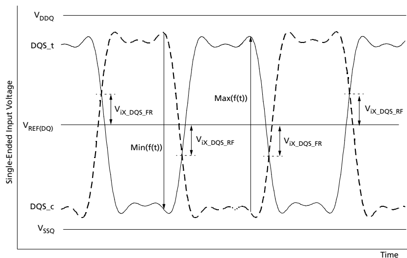
Figure 153: V_{IX} Definition (DQS)
