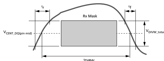
Figure 171: DQ t_{DIPW} and SRIN_dIVW Definition for Each Input Pulse
