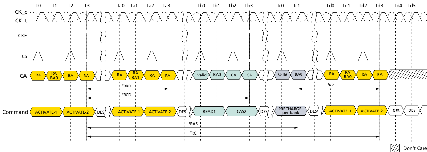
Figure 11: ACTIVATE Command
