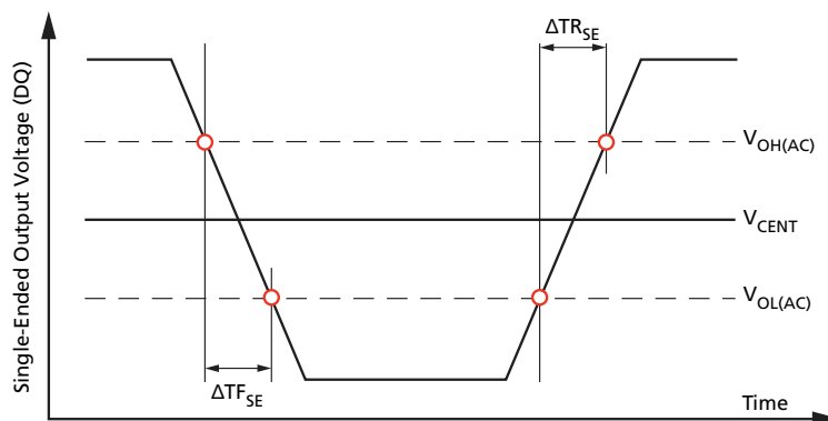
Figure 154: Single-Ended Output Slew Rate Definition
