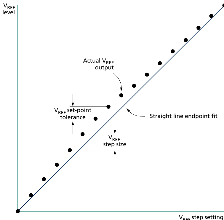
Figure 94: V REF Set-Point Tolerance and Step Size
