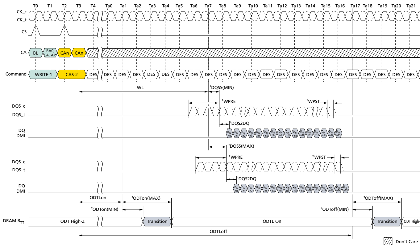
Figure 138: Asynchronous ODTon/ODToff Timing
