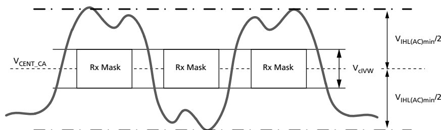
Figure 166: CA V_{IHL\_AC} Definition (for Each Input Pulse)
