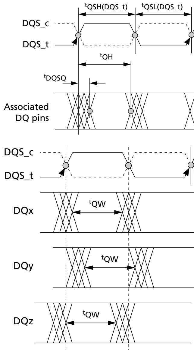
Figure 167: Read Data Timing Definitions – t_{QH} and t_{DQSQ} Across DQ Signals per DQS Group
