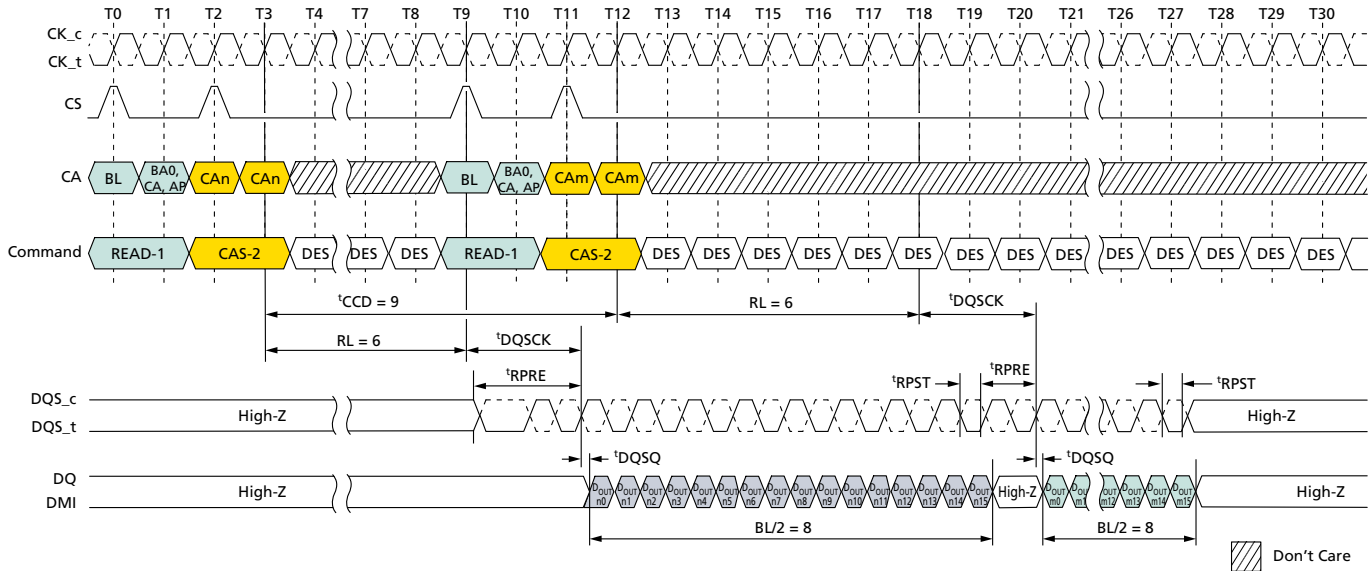
Figure 36: Consecutive READ: t_{CCD} = \text{MIN} + 1 , Preamble = Toggle, 0.5n\text{CK} Postamble
