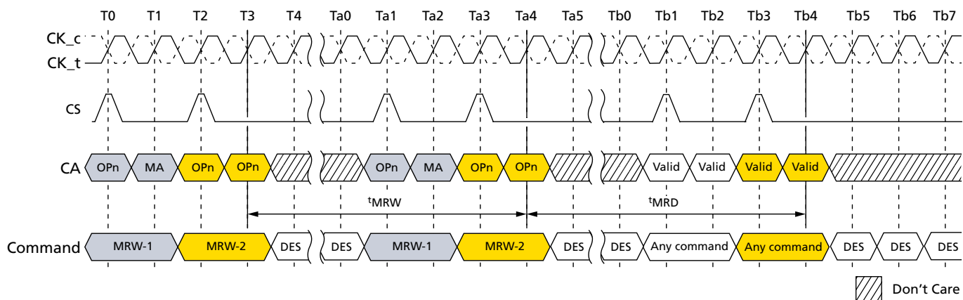
Figure 90: MODE REGISTER WRITE Timing
