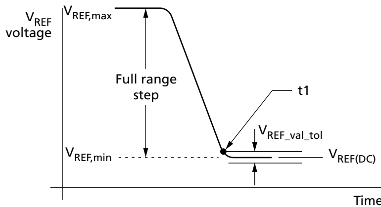
Figure 106: V_{REF(DQ)} Full Step from V_{REF,max} to V_{REF,min}
