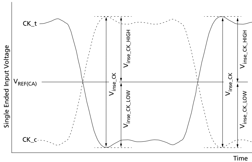
Figure 146: Clock Single-Ended Input Voltage
