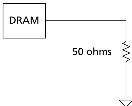
Figure 157: Driver Output Timing Reference Load
