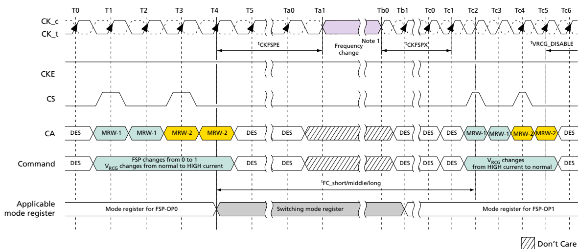
Figure 131: Frequency Set Point Switching Timing
