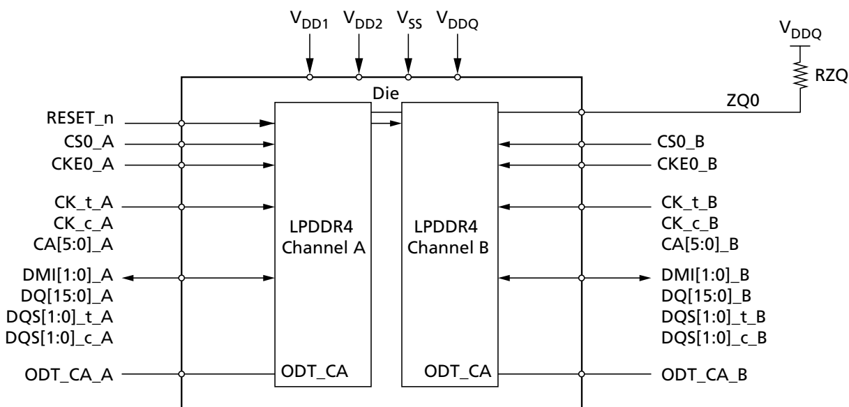
Figure 2: Single-Die, Dual-Channel, Single-Rank Package Block Diagram
