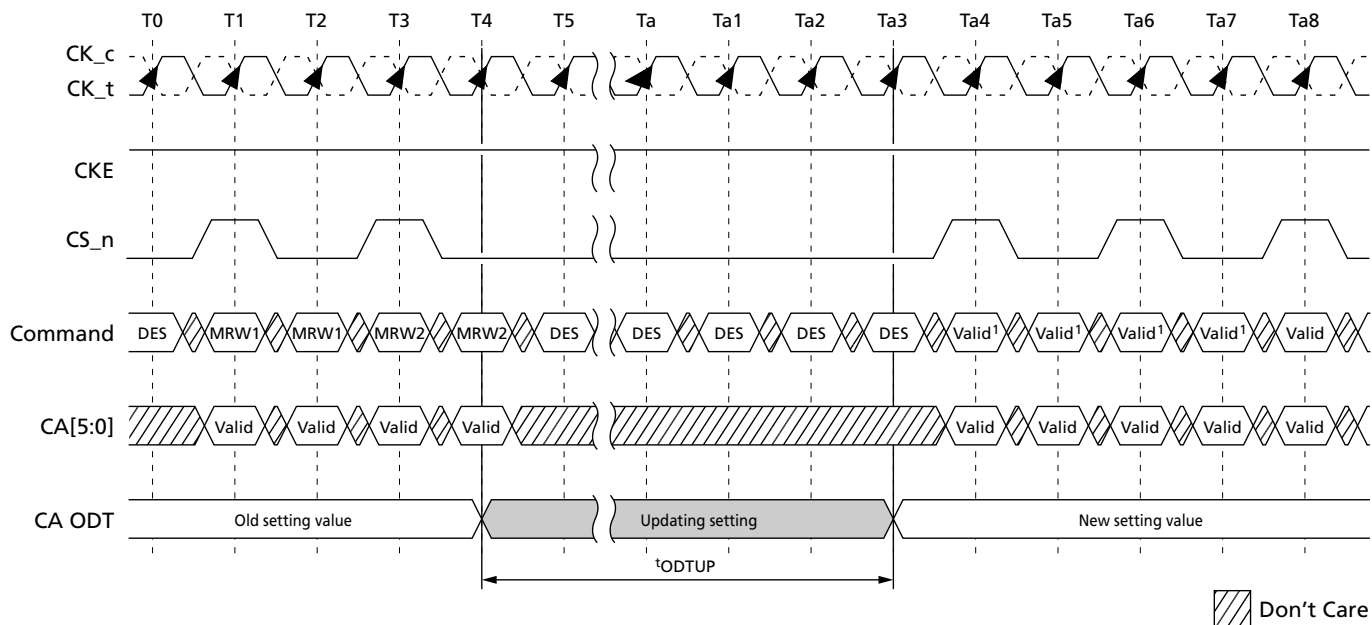
Figure 136: ODT for CA Setting Update Timing in 4-Clock Cycle Command
