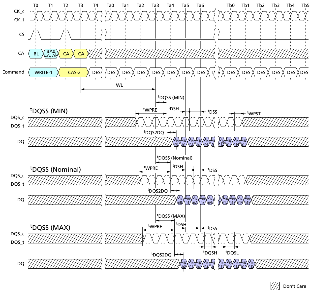
Figure 27: Write Timing
