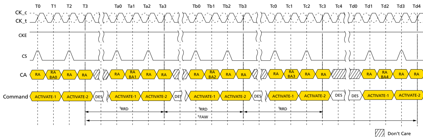
Figure 12: t_{FAW} Timing
