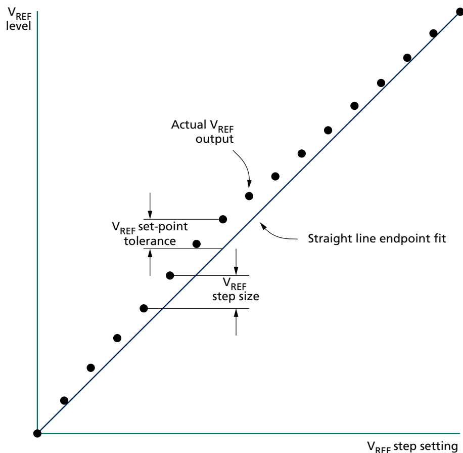
Figure 101: V REF Set Tolerance and Step Size
