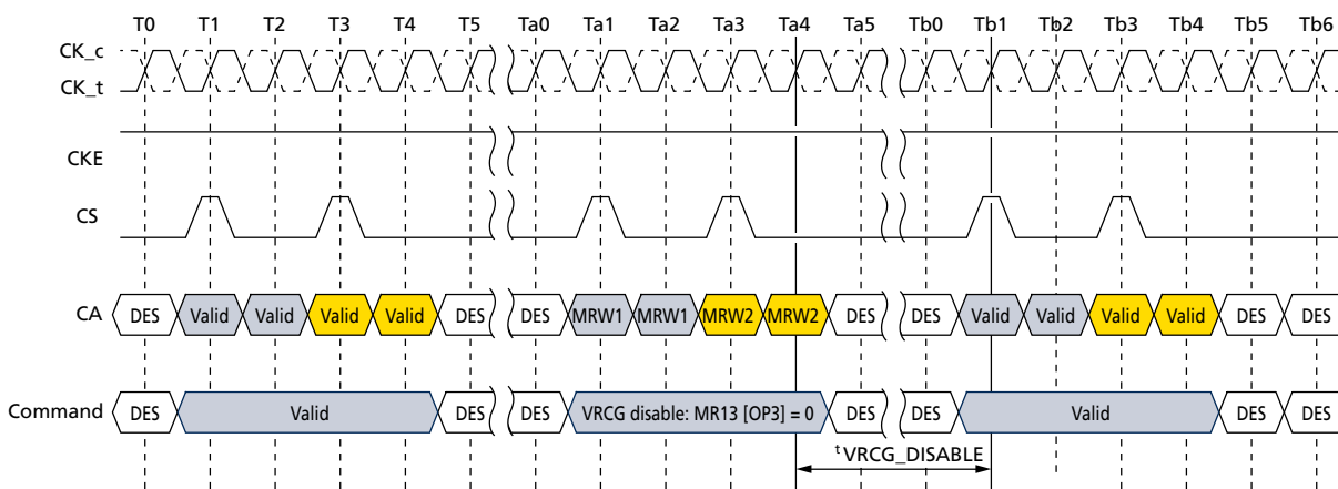
Figure 92: VRCG Disable Timing
