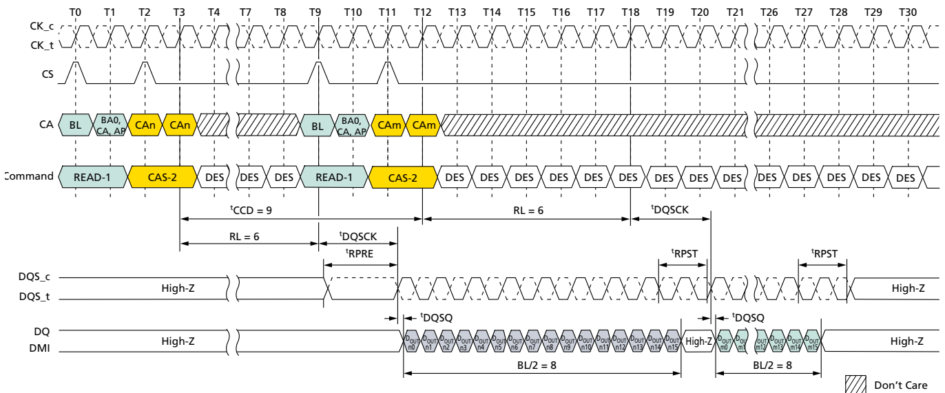
Figure 37: Consecutive READ: t_{CCD} = \text{MIN} + 1 , Preamble = Static, 1.5n\text{CK} Postamble
