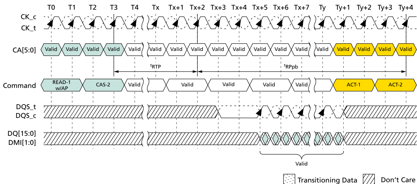
Figure 61: Burst READ With Auto Precharge – BL32, Toggling Preamble, 1.5nCK Postamble
