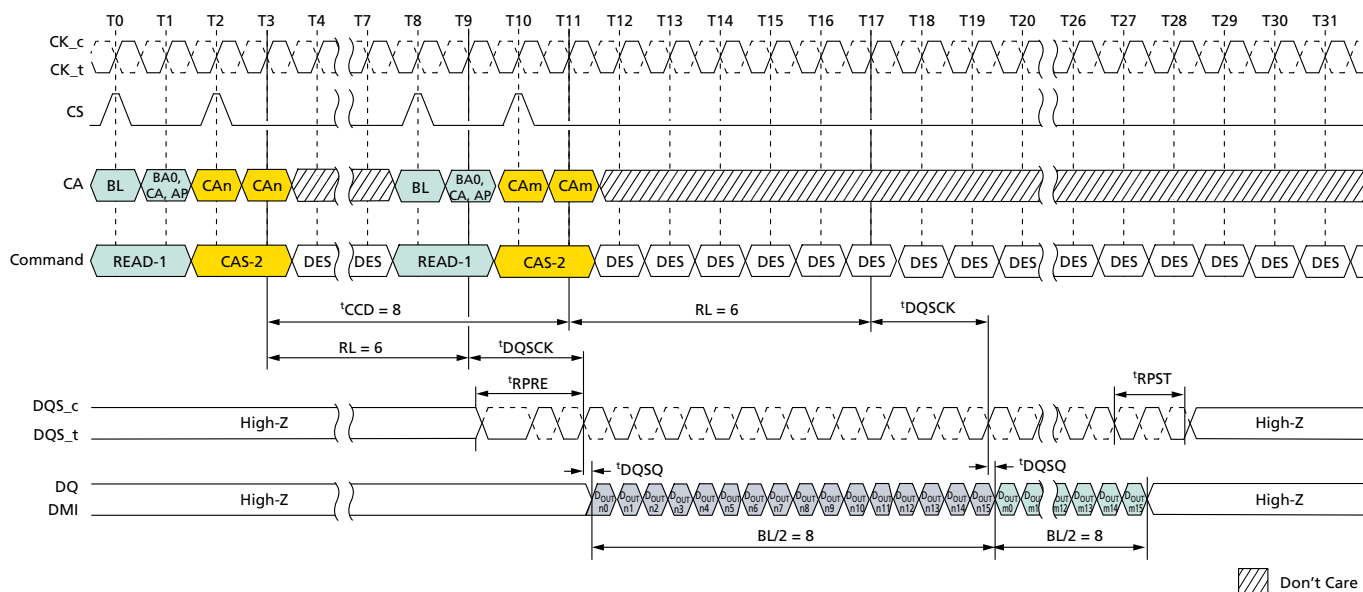
Figure 34: READ Operations: t_{CCD} = \text{MIN} , Preamble = Toggle, 1.5n\text{CK} Postamble
