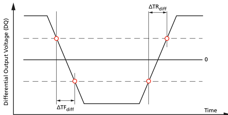
Figure 155: Differential Output Slew Rate Definition
