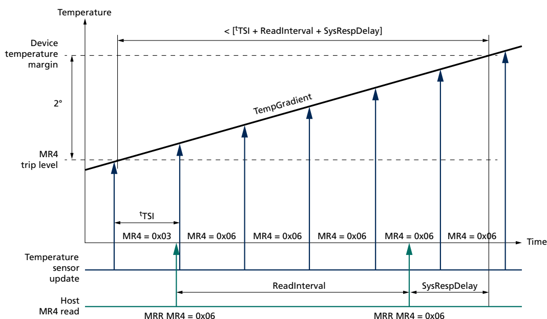
Figure 129: Temperature Sensor Timing
