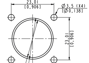
Panel Drilling
