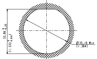
Panel drilling
