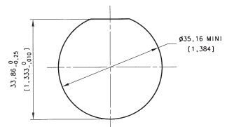
Panel drilling
