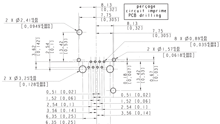
PCB drilling
