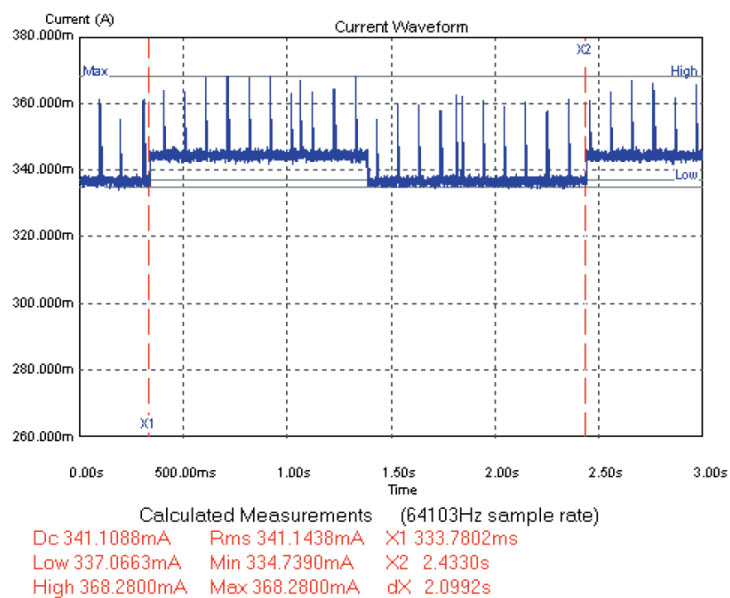
Figure 2. WLAN card idle active current drain waveform capture
