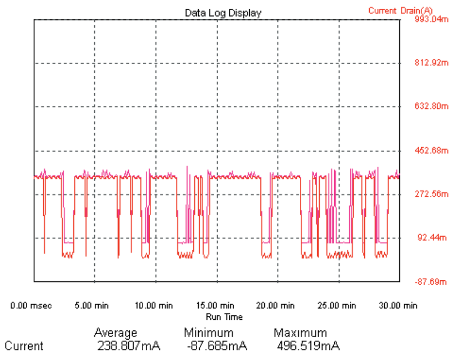
Figure 5. Power savings-on long-term power consumption data log
