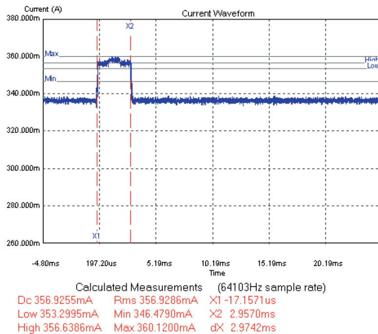
Figure 3. WLAN card transmit beacon current drain pulse
