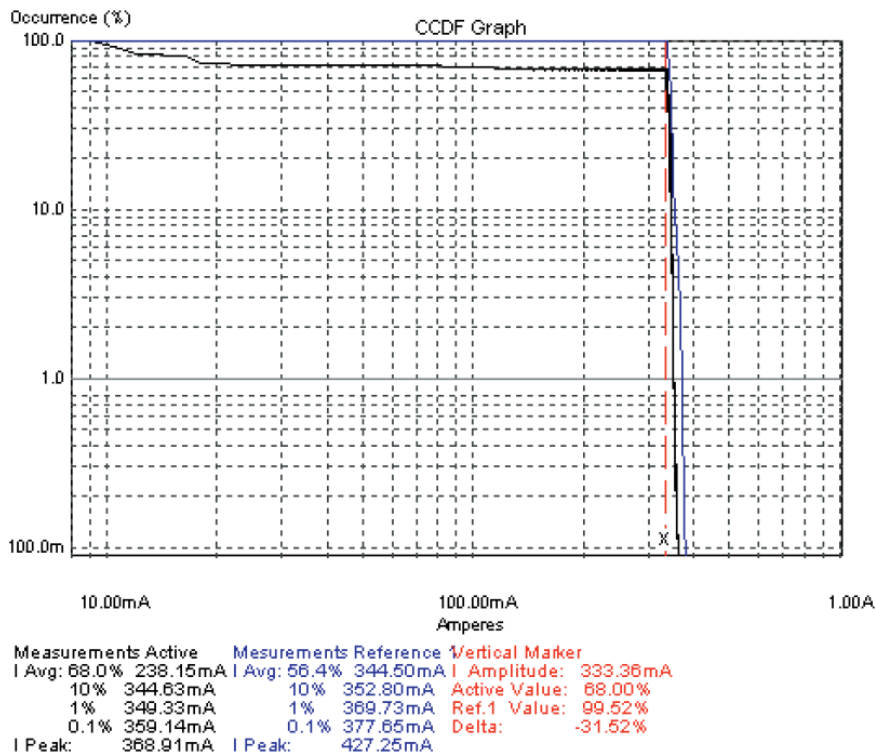
Figure 6. CCDF analysis quantifying power savings gains
