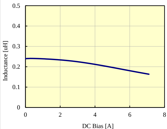
DC Bias vs Inductance
