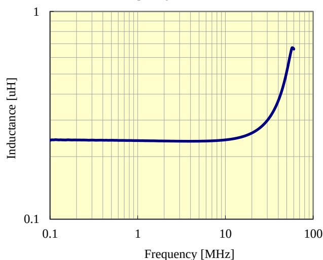
Frequency vs Inductance
