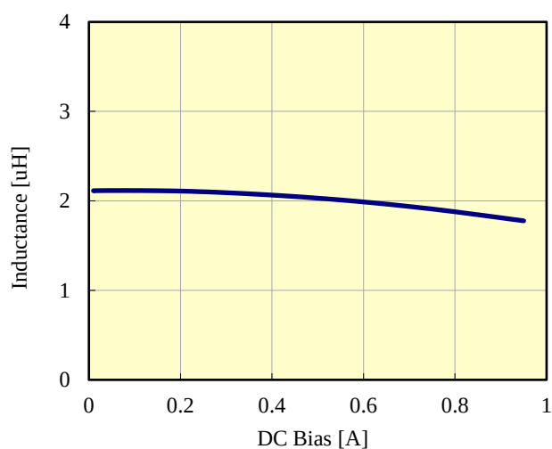
DC Bias vs Inductance
