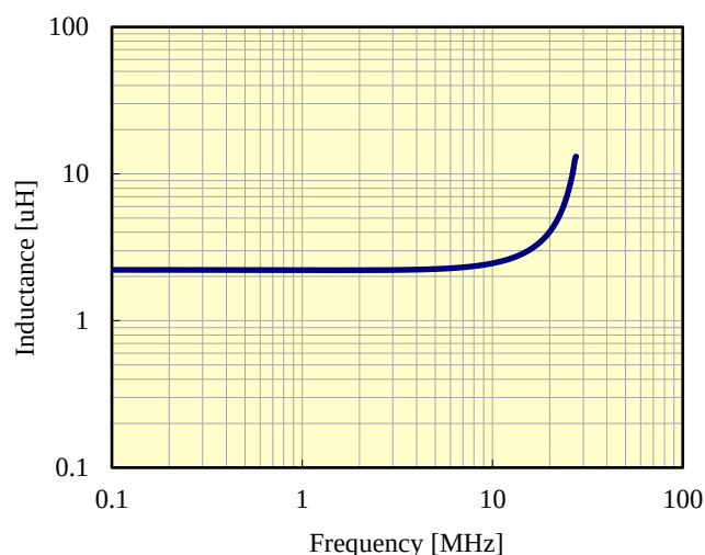
Frequency vs Inductance
