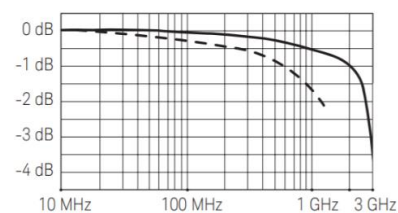
Insertion loss
