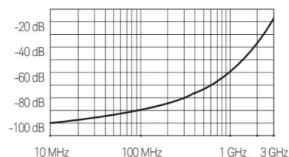
Crosstalk
