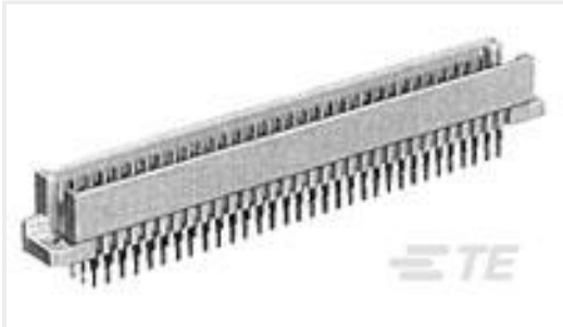
TE Part #650889-5 096 EURO TYPE R PIN AP ASSY
