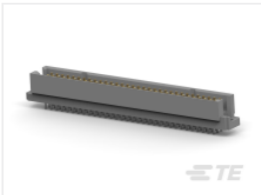
TE Part # 5148304-4 ASSY,PIN,EUROCARD,TYPE R,LEAD-FREE,96 PO
