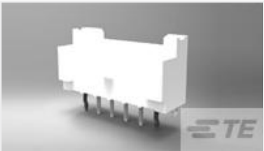
TE Part #1744418-3 3 POS EP 2.5 HDR, GLOW WIRE
