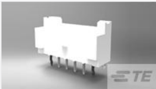
TE Part #1744418-4 4 POS EP 2.5 HDR, GLOW WIRE
