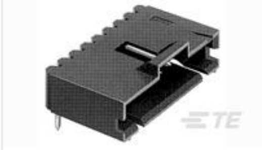
TE Part #6-103635-5 16 MTE HDR SRRA LTCH.100CL LF
