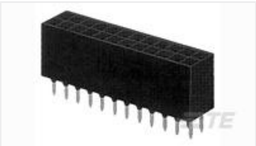
TE Part # 3-534236-0 60 MODII VRT DR CE 100/120
