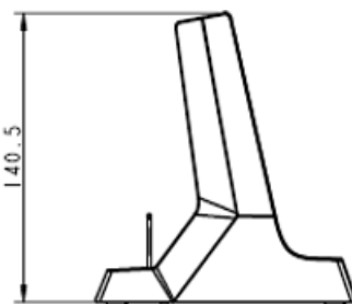
Spare Handle Stand (MP740788)
