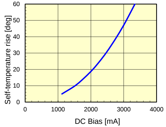
DC Bias vs Temperature
