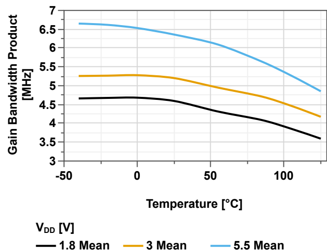
Figure 51-147. Gain Bandwidth Product Over Temperature and V_{DD}
