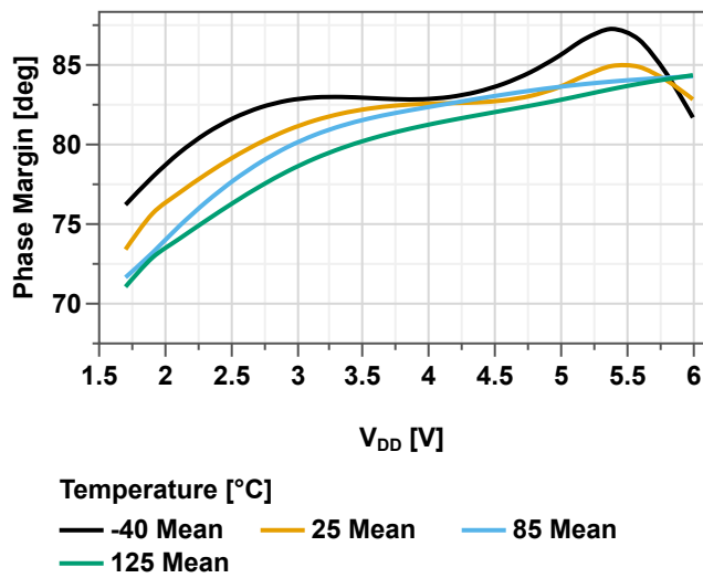
Figure 51-146. Phase Margin Over V_{DD} and Temperature
