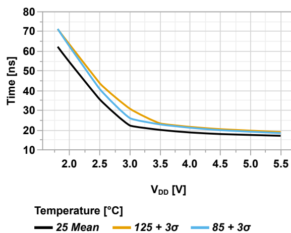
Figure 51-61. Rise Time (SLRxn = b ' 0) vs. V_{DD}
