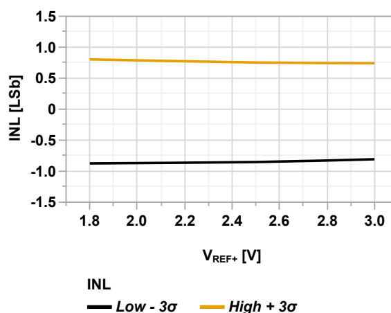
Figure 51-108. INL vs. V_{REF+} (ADC Differential Mode, T_{AD} = 1 \mu s , V_{DD} = 3.0V , T = 25^{\circ}C , CPON = 1 )
