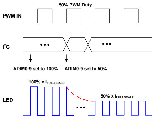
Figure 11: PWM Dimming from PWM Input
