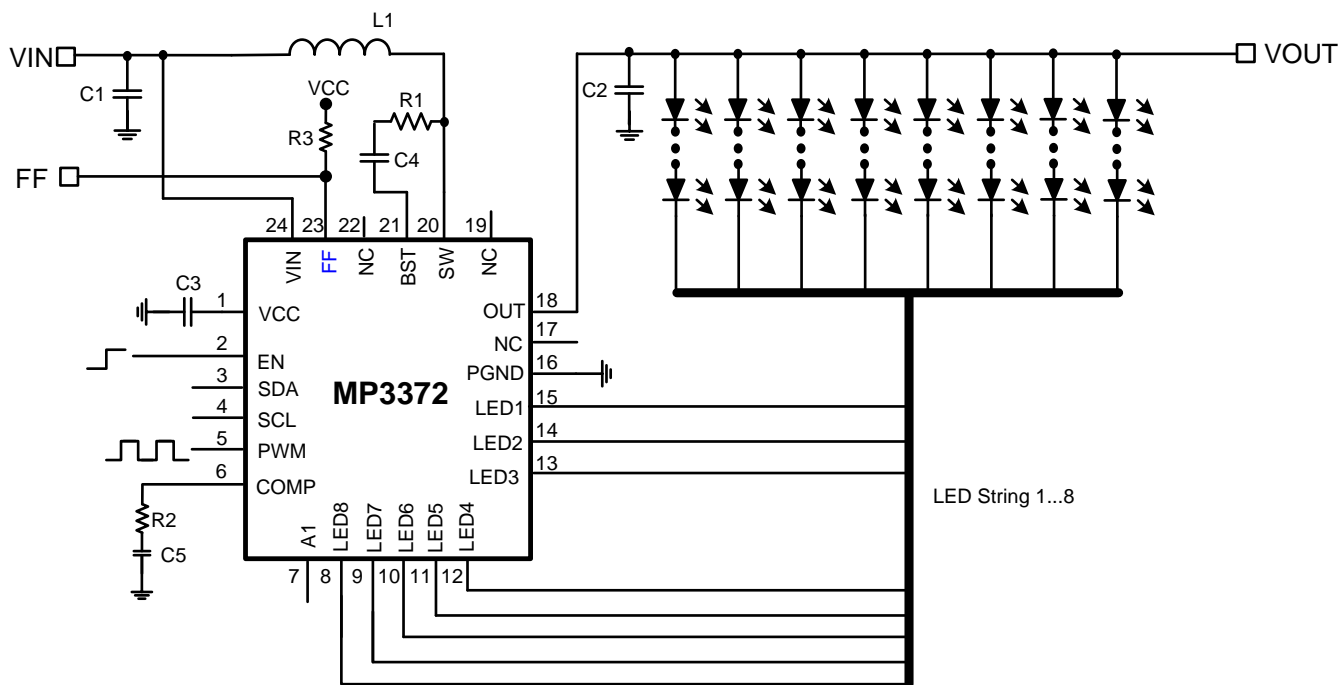
Figure 1: Pull FF to GND when VOUT is Shorted to GND
