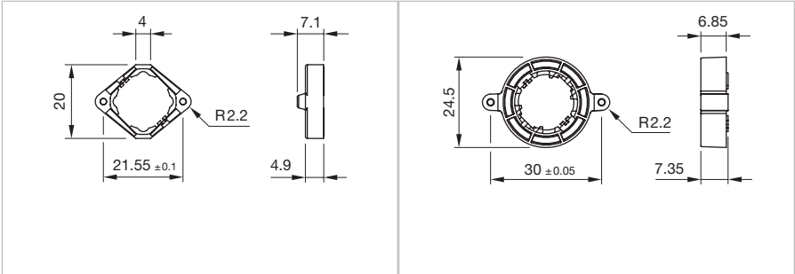
Dimensions [mm] for Part No. 92-960.0
