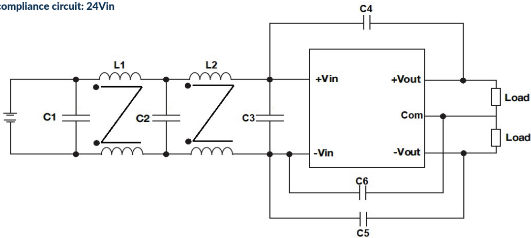
EMC (Class A/B) compliance circuit: 24V in
