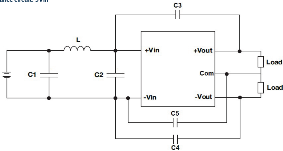
EMC (Class A/B) compliance circuit: 5V in
