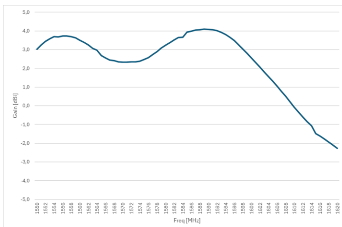
L1 Band
