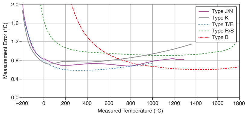
Figure 1. TB-9212 with Mini TC Thermocouple Error Typical (High-Speed), 23 °C ±5 °C
