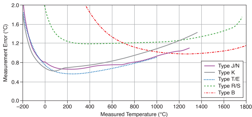
Figure 1. TB-9212 with Mini TC Thermocouple Error Maximum (High-Speed), -20 °C to 70 °C
