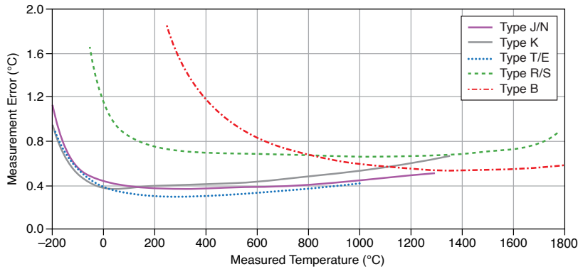
Figure 1. TB-9212 with Mini TC Thermocouple Error Typical (High-Resolution, Best 50/60 Hz Rejection), 23 °C ±5 °C
