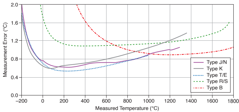
Figure 1. TB-9212 with Screw Terminal Thermocouple Error Maximum (High-Speed), -20 °C to 70 °C
