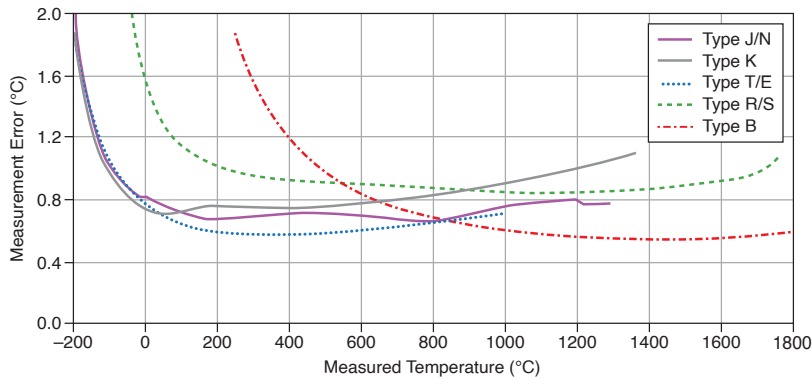
Figure 1. TB-9212 with Screw Terminal Thermocouple Error Typical (High-Speed), 23 °C ±5 °C
