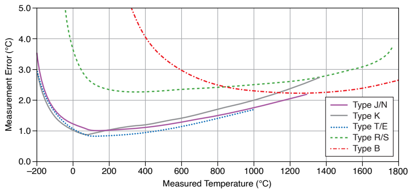
Figure 1. TB-9212 with Mini TC Thermocouple Error Maximum (High-Resolution, Best 50/60 Hz Rejection), -20 °C to 70 °C
