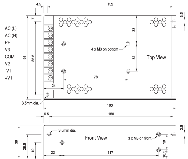
PBC60W TRIPLE
