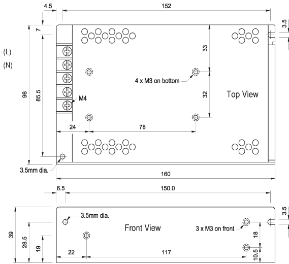
PBC70W SINGLE
