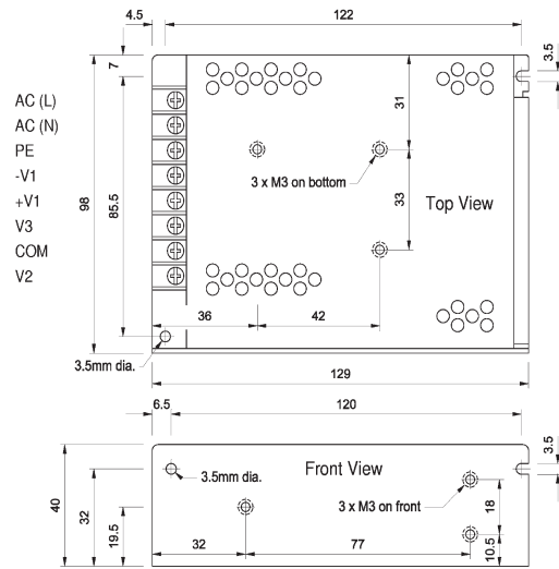
PBC60W TRIPLE
