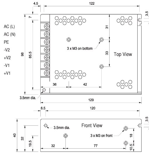
PBC40W DUAL
