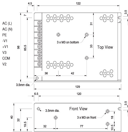
PBC50W TRIPLE
