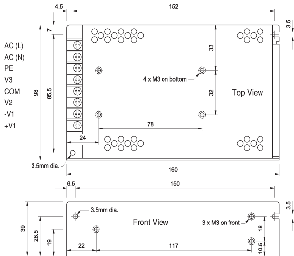
PBC50W TRIPLE
