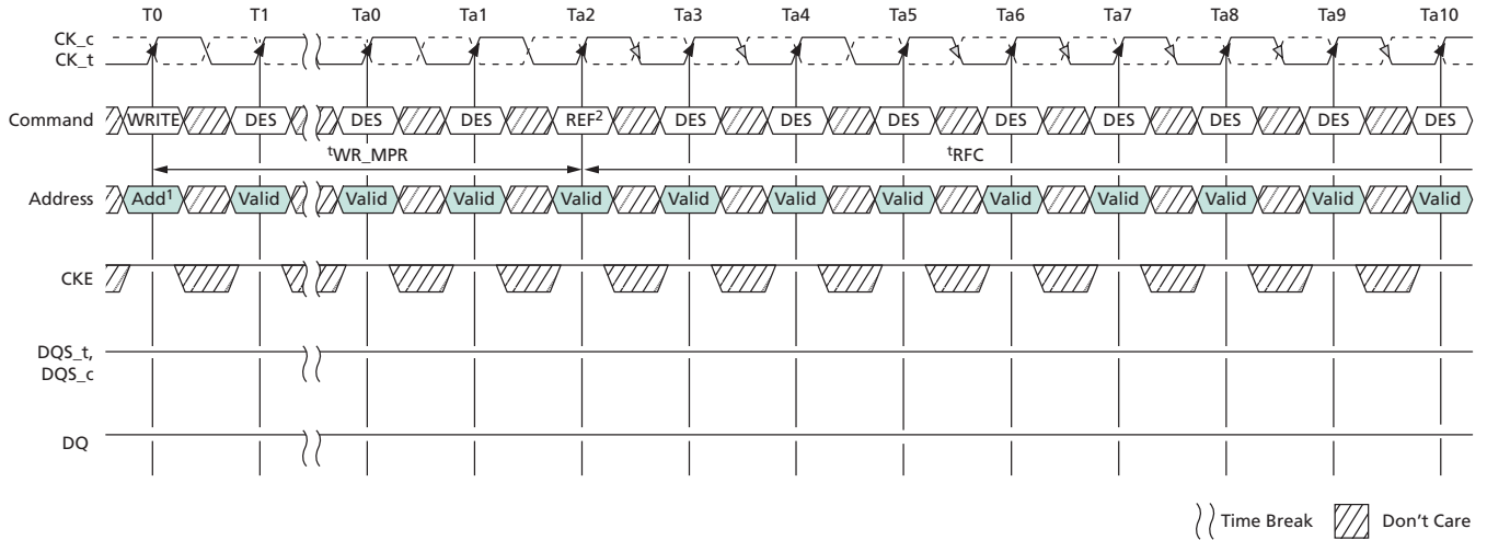
Figure 42: WRITE-to-REFRESH Timing
