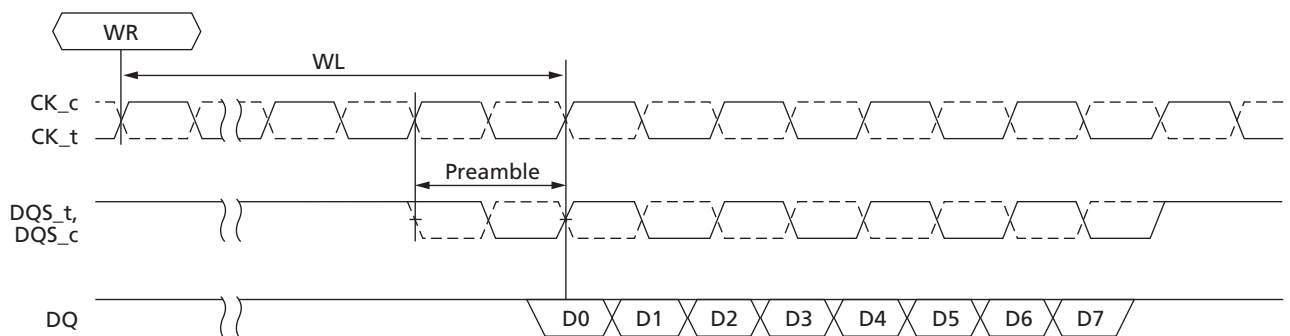
Figure 110: 1^t\text{CK} vs. 2^t\text{CK} WRITE Preamble Mode
