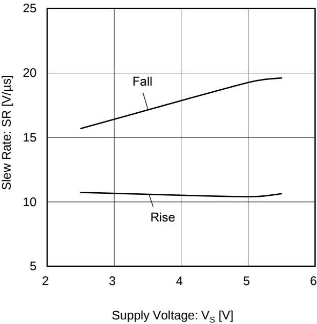
Figure 19. Slew Rate vs Supply Voltage
