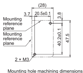
Mounting hole machining dimensions
