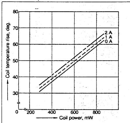
Without diode (T 2 )
