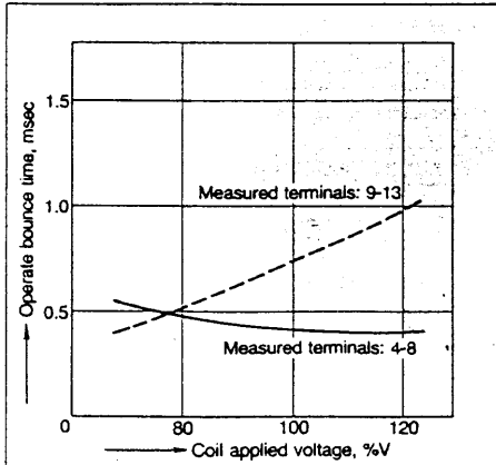
Without diode (T 2 )
