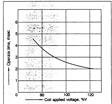
Without diode (T 4 )
