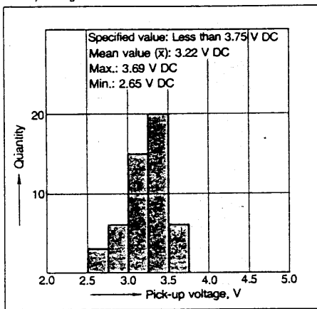
Pick-up voltage
