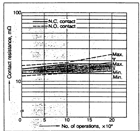
Without diode (T 1 )
