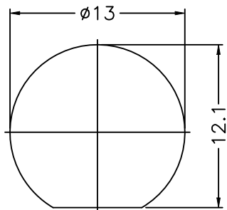
RECOMMENDED MOUNTING HOLE MAX. PANEL THICKNESS=6mm
