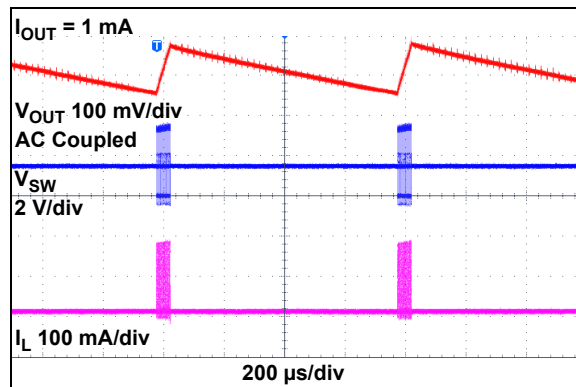
FIGURE 2-18: MCP16251 3.3V_{OUT} PFM Mode Waveforms.
