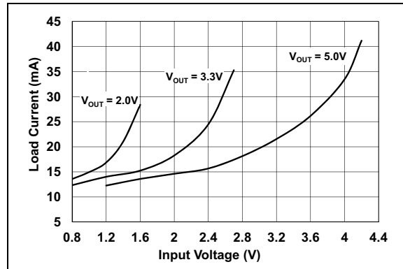
FIGURE 2-17: Average of PFM-to-PWM Threshold Current vs. V_{IN} .
