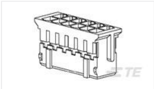
TE Part #1-1470107-6 2.0MM PITCH CRIMP HOUSING 16P
