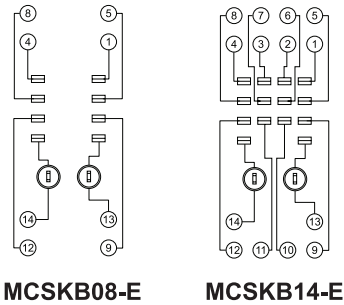
Wiring Diagram
