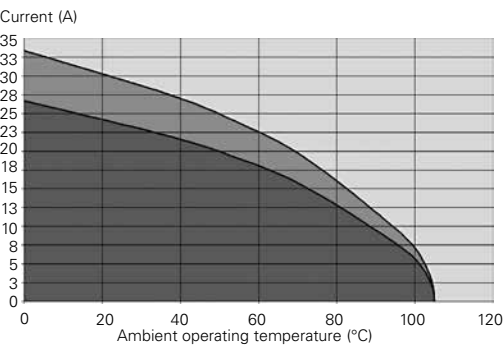
Fig.3: UTO 12-4 – Wire section 20 AWG
