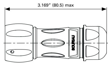
Fig. 5 : Cable diameter acceptance from 0.275" to 0.393" (7 to 10)
