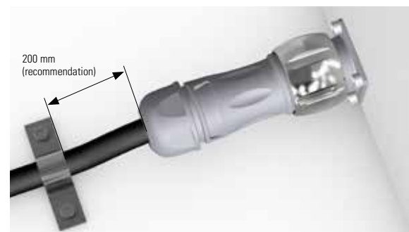
6 - Example of installation
