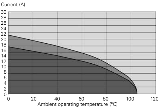
Fig.2: UTO 12-8 – Wire section 16 AWG
