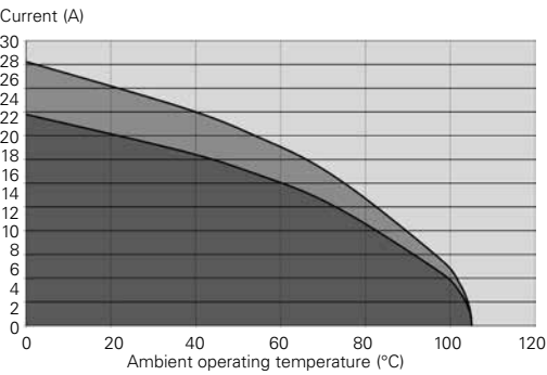
Fig.1: UTO 12-4 – Wire section 16 AWG
