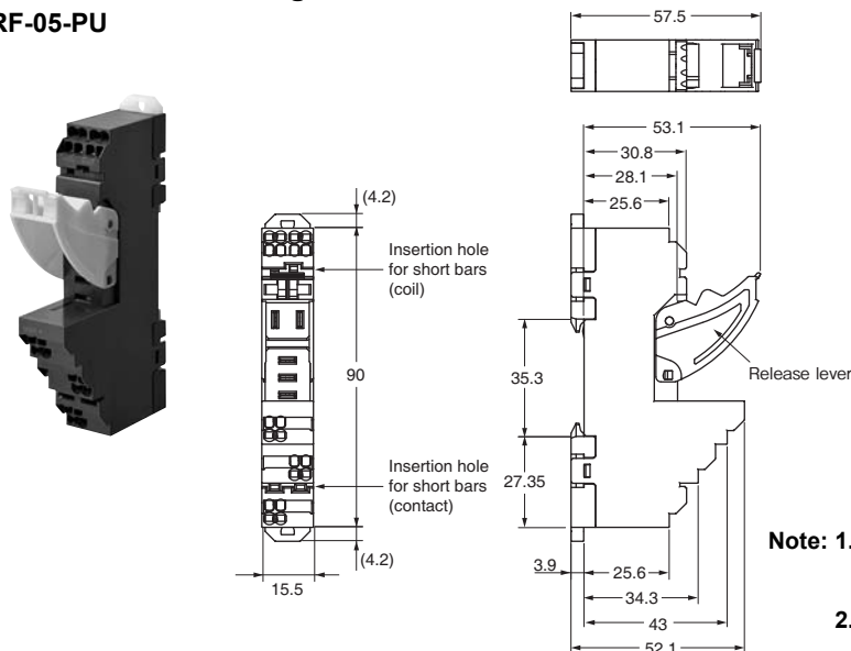
Terminal Arrangement/ Internal Connection Diagram (Top View)
