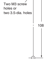
Mounting Hole Dimensions
