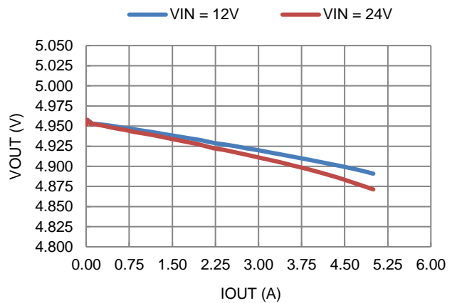
Figure 7. Load Regulation
