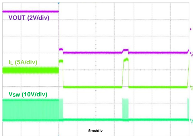
Figure 21. Output Short Protection, I_{OUT} = 5\text{A}
