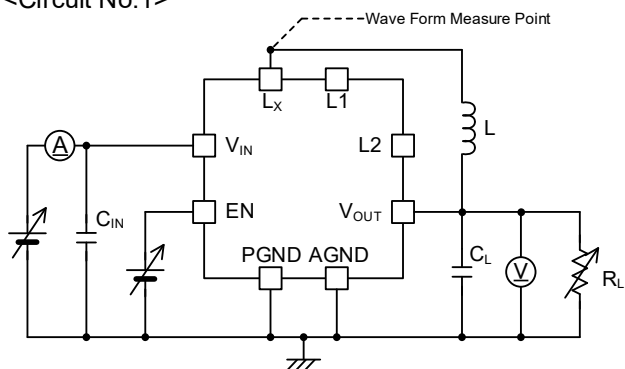
<Circuit No.1>
