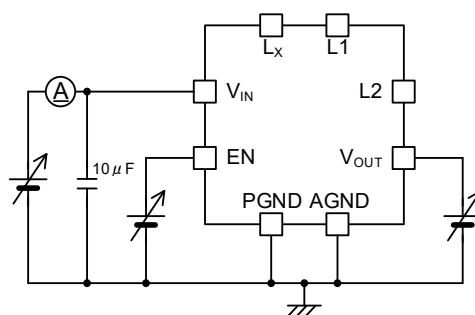
<Circuit No.2>
